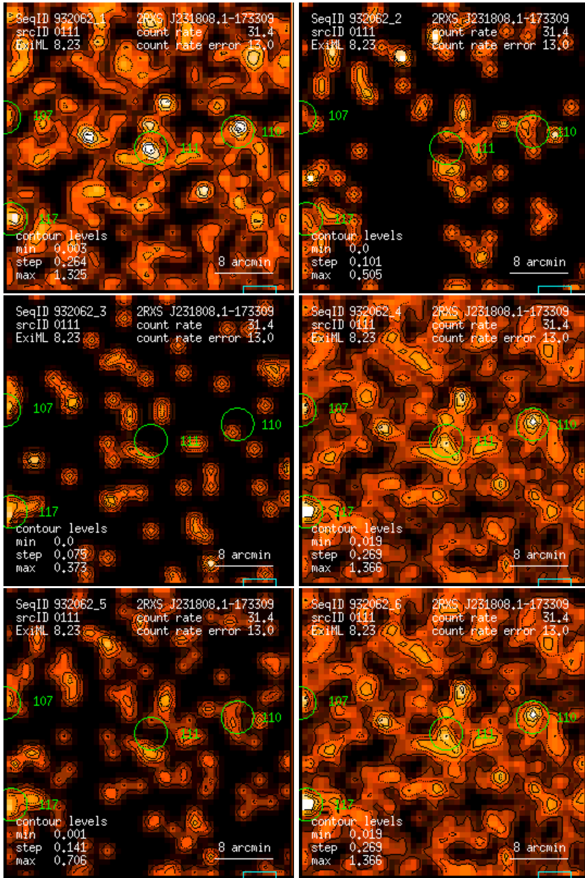
Figure 111: RASS 932062: detection 0111: band rate images, Gaussian filter: (1) PSPC channels 11 – 41, (2) 52 – 90, (3) 91 – 201, (4) 11 – 235, (5) 52 – 201, (6) 11 – 201. Broad band rates in counts/ks. Band rate contour levels in counts/ks/arcmin 2 .
