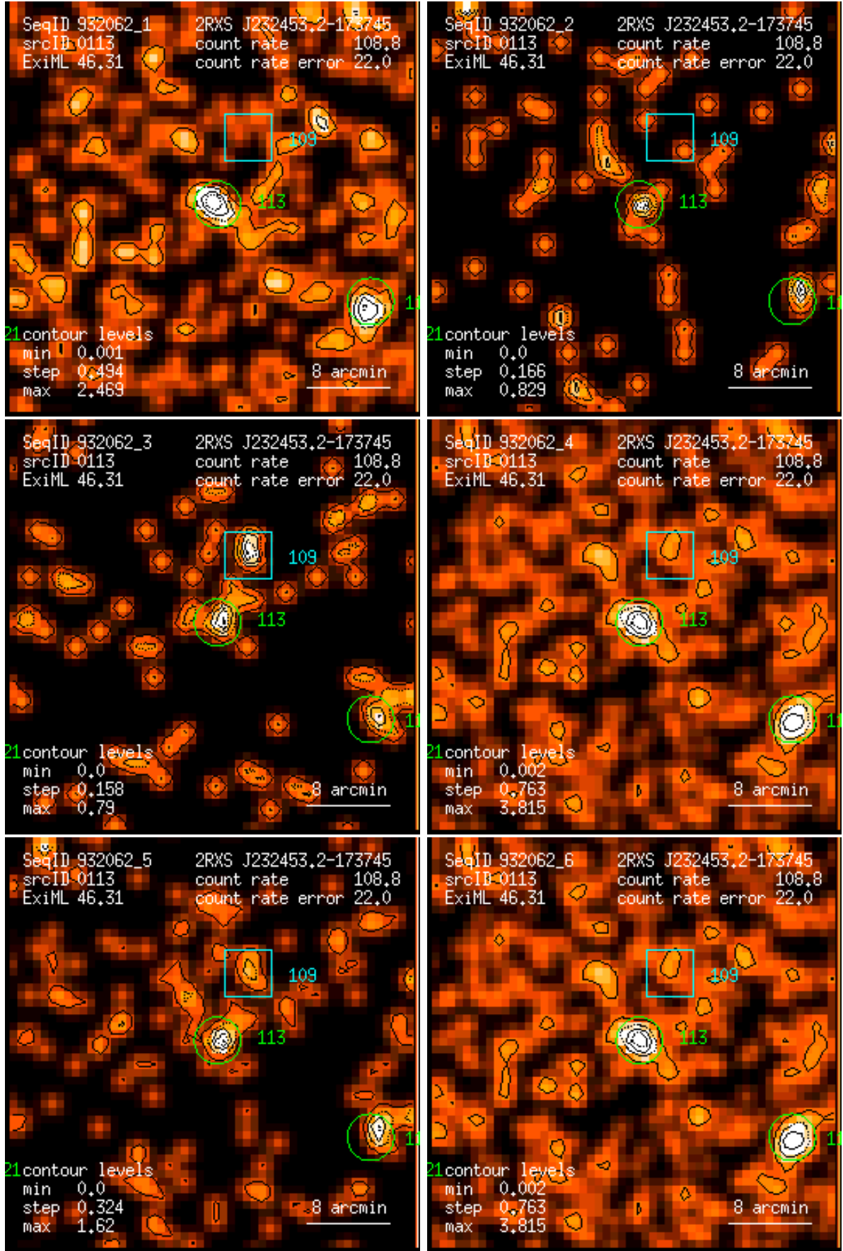
Figure 113: RASS 932062: detection 0113: band rate images, Gaussian filter: (1) PSPC channels 11 – 41, (2) 52 – 90, (3) 91 – 201, (4) 11 – 235, (5) 52 – 201, (6) 11 – 201. Broad band rates in counts/ks. Band rate contour levels in counts/ks/arcmin 2 .
