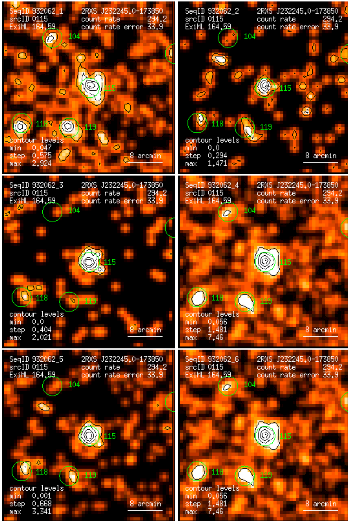
Figure 115: RASS 932062: detection 0115: band rate images, Gaussian filter: (1) PSPC channels 11 – 41, (2) 52 – 90, (3) 91 – 201, (4) 11 – 235, (5) 52 – 201, (6) 11 – 201. Broad band rates in counts/ks. Band rate contour levels in counts/ks/arcmin 2 .
