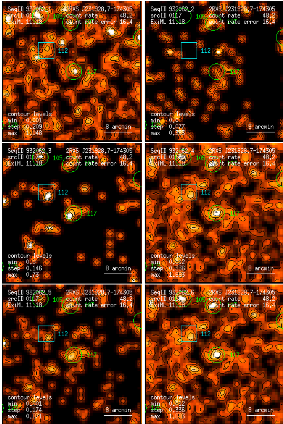
Figure 117: RASS 932062: detection 0117: band rate images, Gaussian filter: (1) PSPC channels 11 – 41, (2) 52 – 90, (3) 91 – 201, (4) 11 – 235, (5) 52 – 201, (6) 11 – 201. Broad band rates in counts/ks. Band rate contour levels in counts/ks/arcmin 2 .
