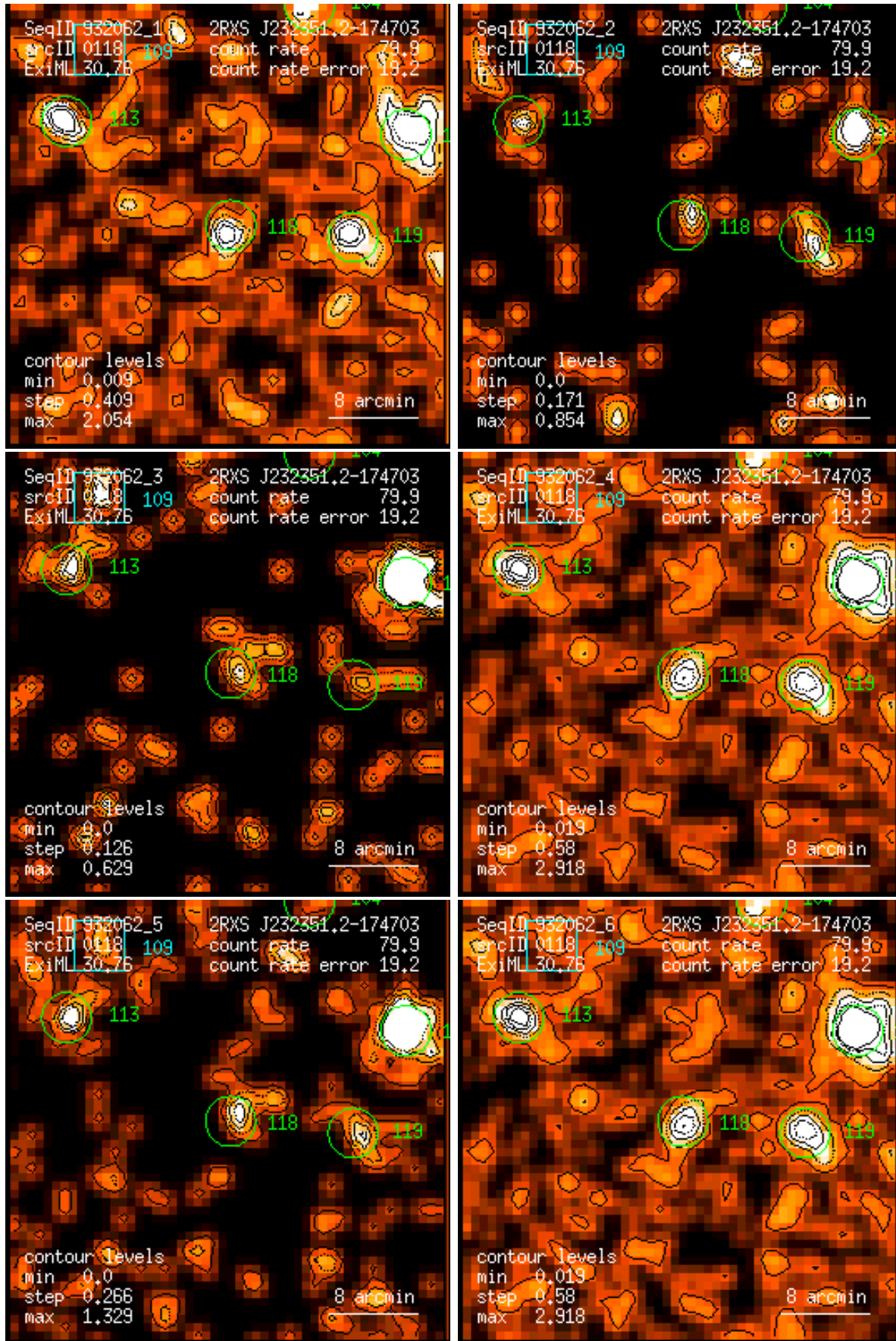
Figure 118: RASS 932062: detection 0118: band rate images, Gaussian filter: (1) PSPC channels 11 – 41, (2) 52 – 90, (3) 91 – 201, (4) 11 – 235, (5) 52 – 201, (6) 11 – 201. Broad band rates in counts/ks. Band rate contour levels in counts/ks/arcmin 2 .
