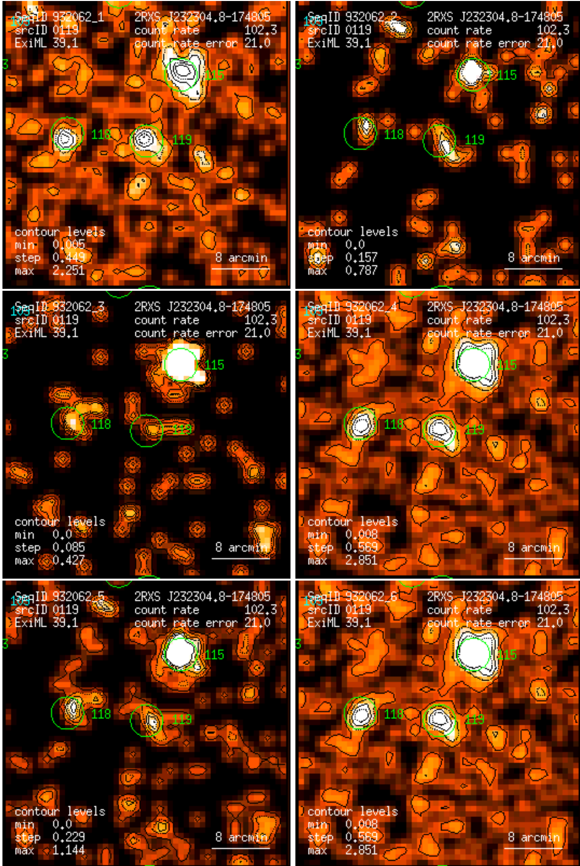
Figure 119: RASS 932062: detection 0119: band rate images, Gaussian filter: (1) PSPC channels 11 – 41, (2) 52 – 90, (3) 91 – 201, (4) 11 – 235, (5) 52 – 201, (6) 11 – 201. Broad band rates in counts/ks. Band rate contour levels in counts/ks/arcmin 2 .
