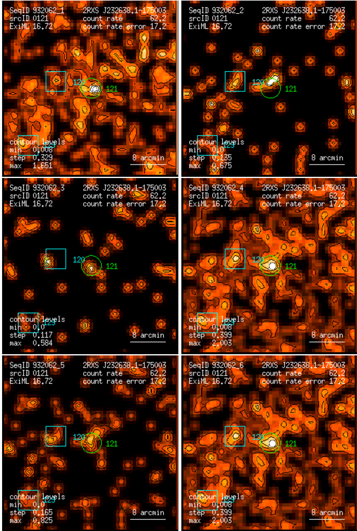
Figure 121: RASS 932062: detection 0121: band rate images, Gaussian filter: (1) PSPC channels 11 – 41, (2) 52 – 90, (3) 91 – 201, (4) 11 – 235, (5) 52 – 201, (6) 11 – 201. Broad band rates in counts/ks. Band rate contour levels in counts/ks/arcmin 2 .
