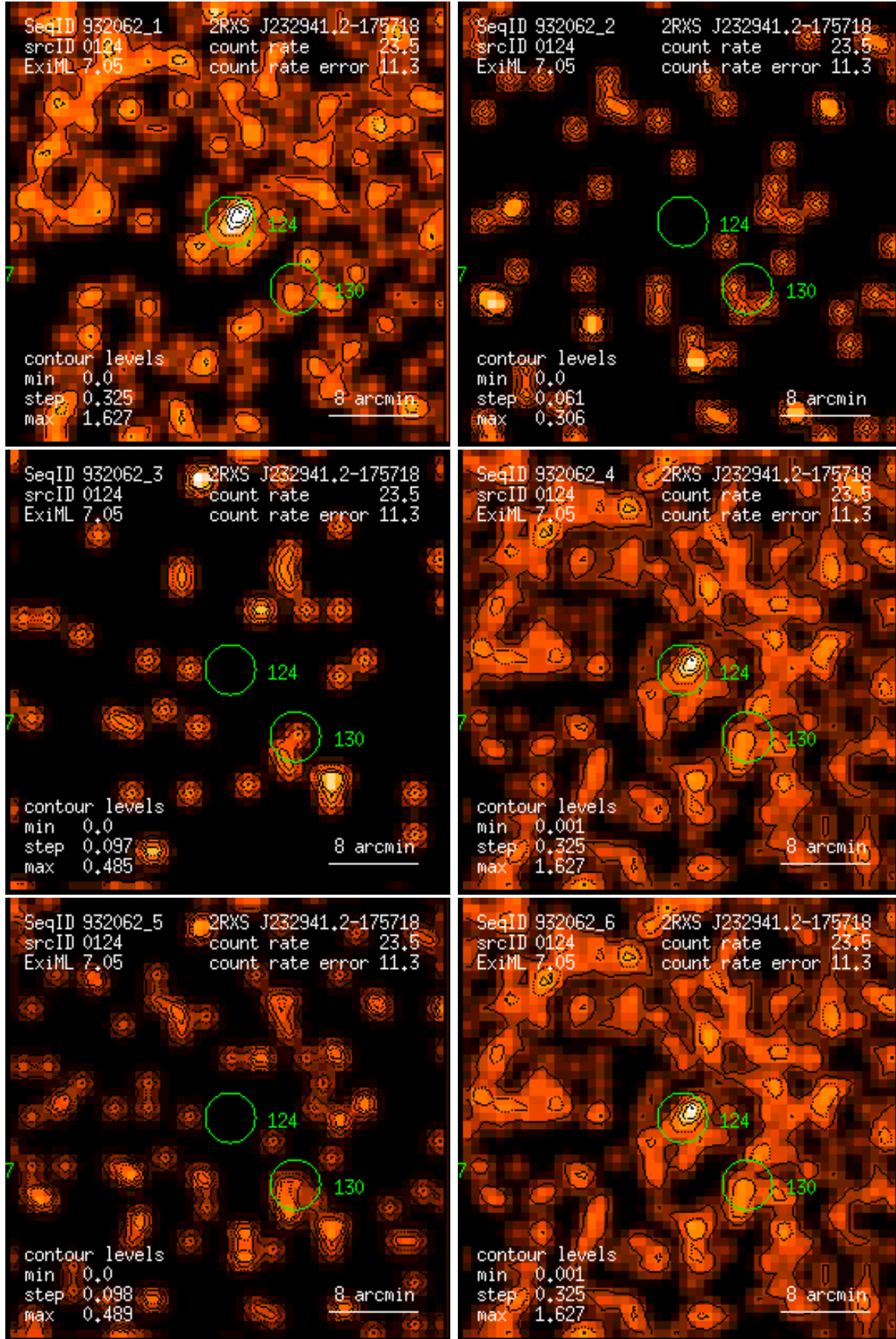
Figure 124: RASS 932062: detection 0124: band rate images, Gaussian filter: (1) PSPC channels 11 – 41, (2) 52 – 90, (3) 91 – 201, (4) 11 – 235, (5) 52 – 201, (6) 11 – 201. Broad band rates in counts/ks. Band rate contour levels in counts/ks/arcmin 2 .
