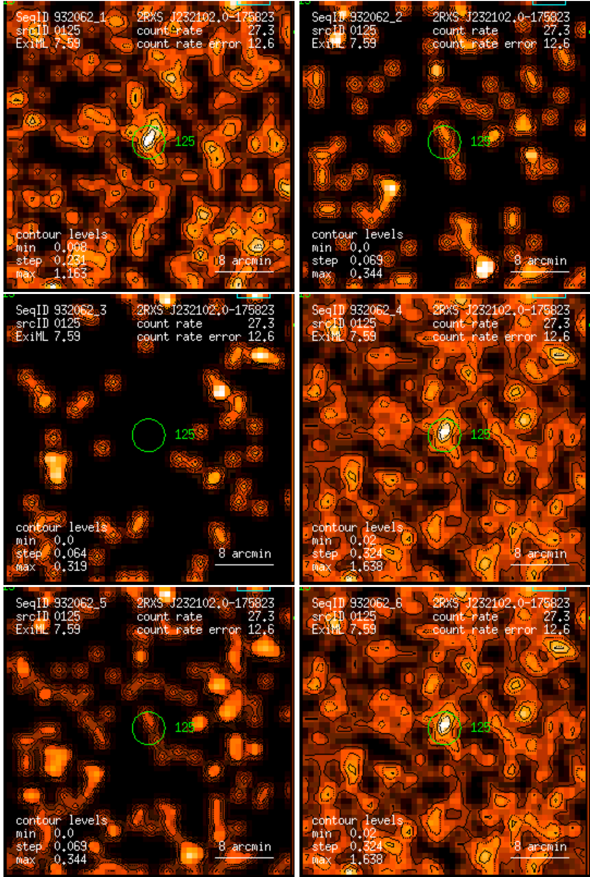
Figure 125: RASS 932062: detection 0125: band rate images, Gaussian filter: (1) PSPC channels 11 – 41, (2) 52 – 90, (3) 91 – 201, (4) 11 – 235, (5) 52 – 201, (6) 11 – 201. Broad band rates in counts/ks. Band rate contour levels in counts/ks/arcmin 2 .
