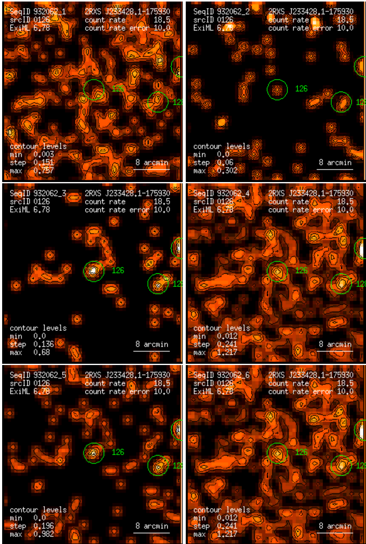
Figure 126: RASS 932062: detection 0126: band rate images, Gaussian filter: (1) PSPC channels 11 – 41, (2) 52 – 90, (3) 91 – 201, (4) 11 – 235, (5) 52 – 201, (6) 11 – 201. Broad band rates in counts/ks. Band rate contour levels in counts/ks/arcmin 2 .
