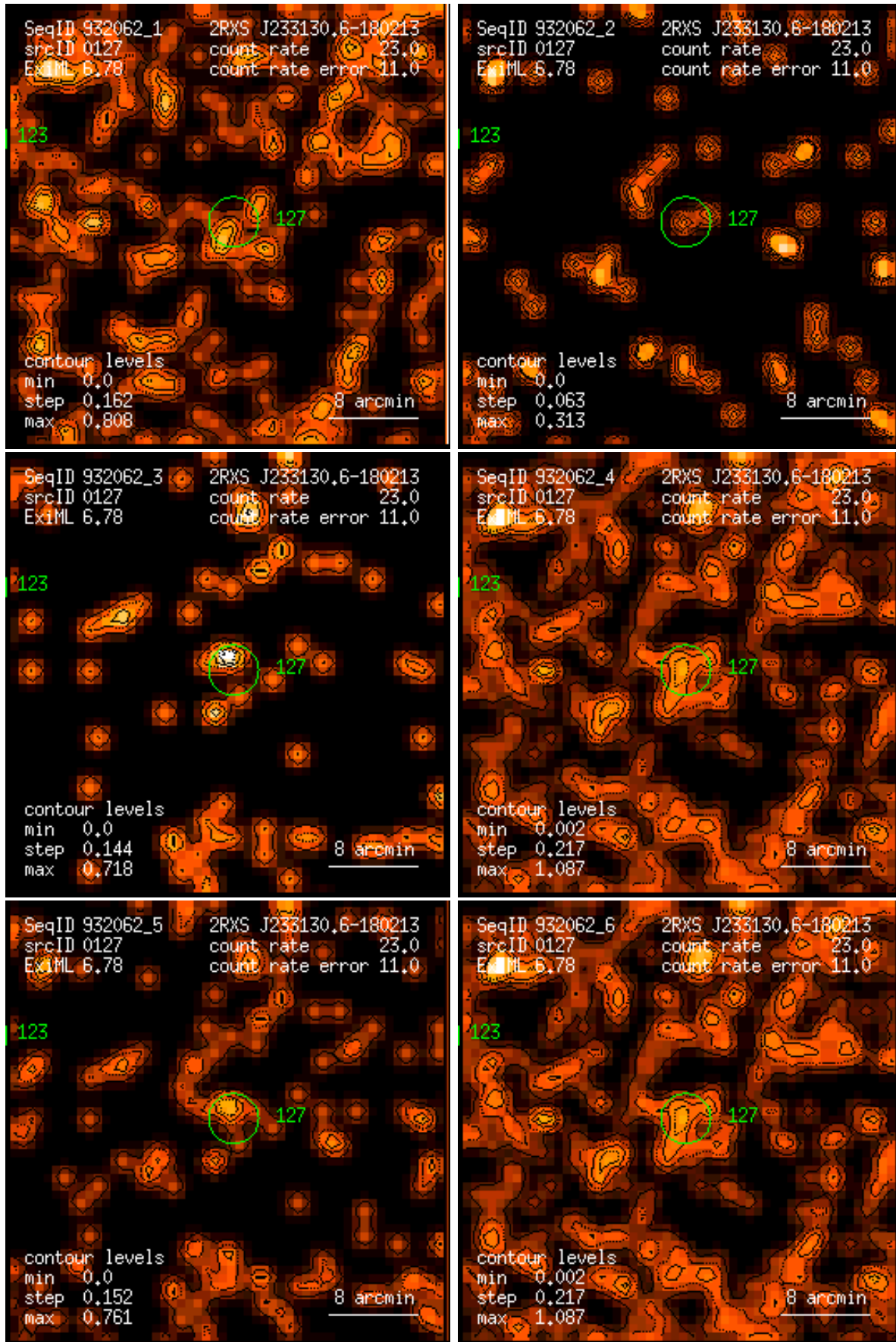
Figure 127: RASS 932062: detection 0127: band rate images, Gaussian filter: (1) PSPC channels 11 – 41, (2) 52 – 90, (3) 91 – 201, (4) 11 – 235, (5) 52 – 201, (6) 11 – 201. Broad band rates in counts/ks. Band rate contour levels in counts/ks/arcmin 2 .
