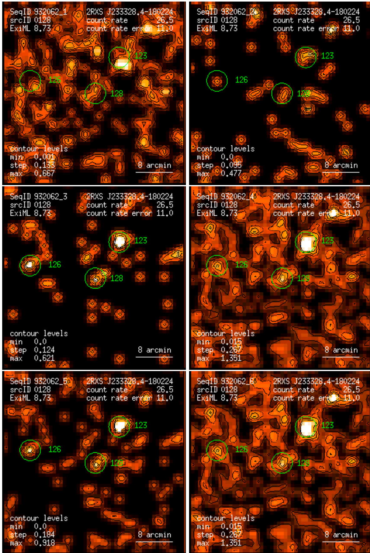
Figure 128: RASS 932062: detection 0128: band rate images, Gaussian filter: (1) PSPC channels 11 – 41, (2) 52 – 90, (3) 91 – 201, (4) 11 – 235, (5) 52 – 201, (6) 11 – 201. Broad band rates in counts/ks. Band rate contour levels in counts/ks/arcmin 2 .
