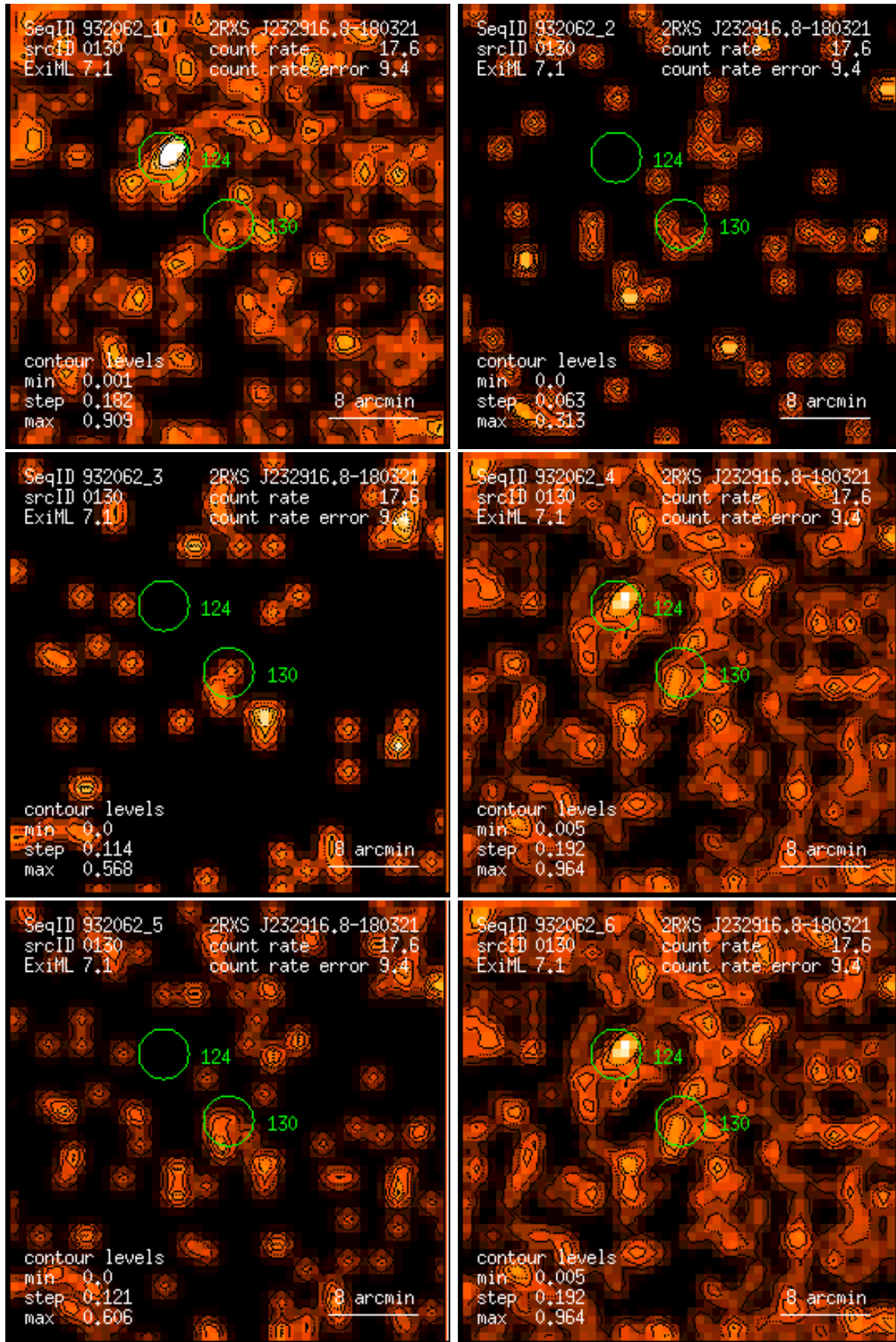
Figure 130: RASS 932062: detection 0130: band rate images, Gaussian filter: (1) PSPC channels 11 – 41, (2) 52 – 90, (3) 91 – 201, (4) 11 – 235, (5) 52 – 201, (6) 11 – 201. Broad band rates in counts/ks. Band rate contour levels in counts/ks/arcmin 2 .
