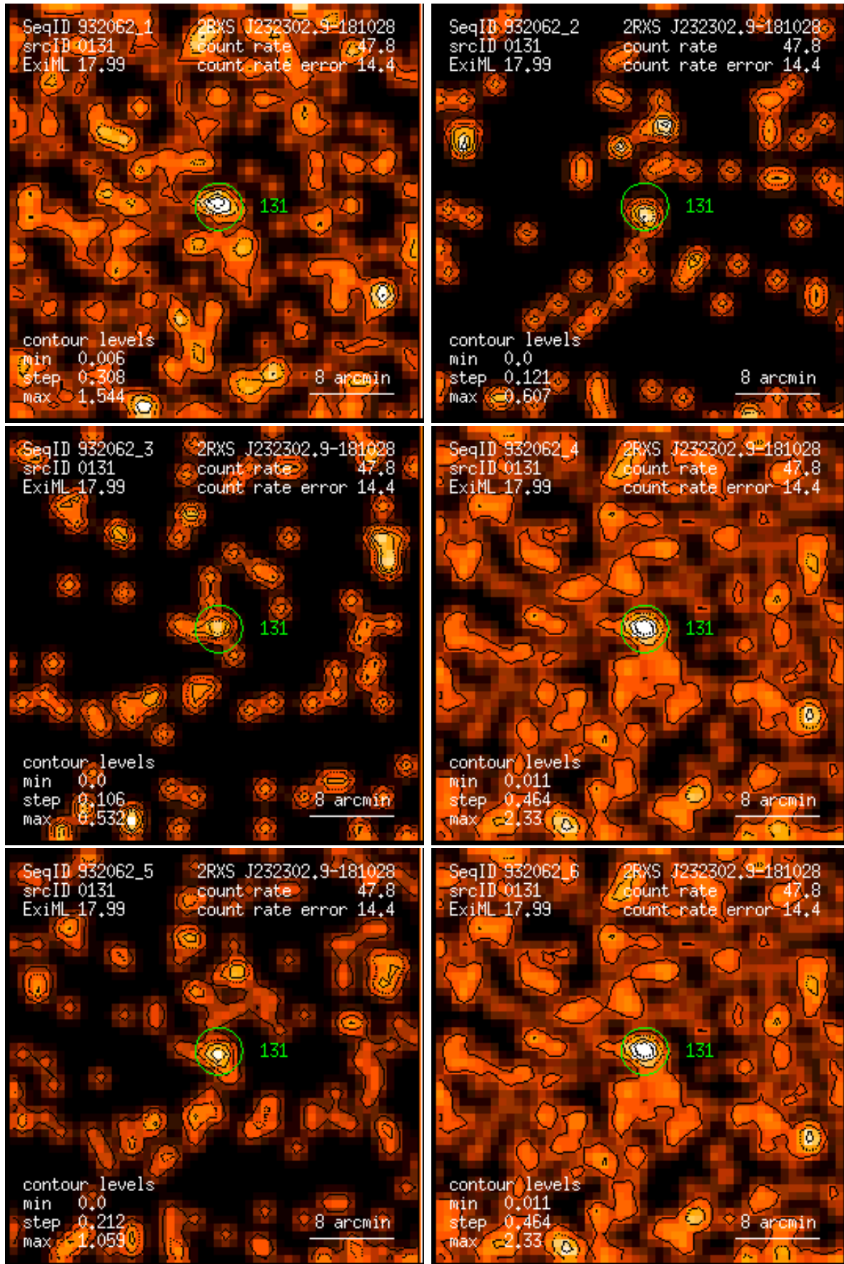
Figure 131: RASS 932062: detection 0131: band rate images, Gaussian filter: (1) PSPC channels 11 – 41, (2) 52 – 90, (3) 91 – 201, (4) 11 – 235, (5) 52 – 201, (6) 11 – 201. Broad band rates in counts/ks. Band rate contour levels in counts/ks/arcmin 2 .
