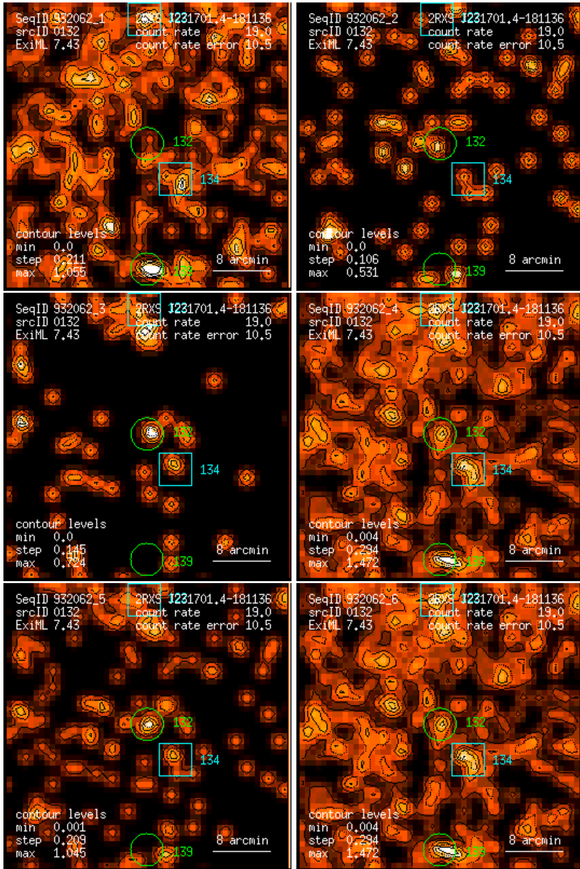
Figure 132: RASS 932062: detection 0132: band rate images, Gaussian filter: (1) PSPC channels 11 – 41, (2) 52 – 90, (3) 91 – 201, (4) 11 – 235, (5) 52 – 201, (6) 11 – 201. Broad band rates in counts/ks. Band rate contour levels in counts/ks/arcmin 2 .
