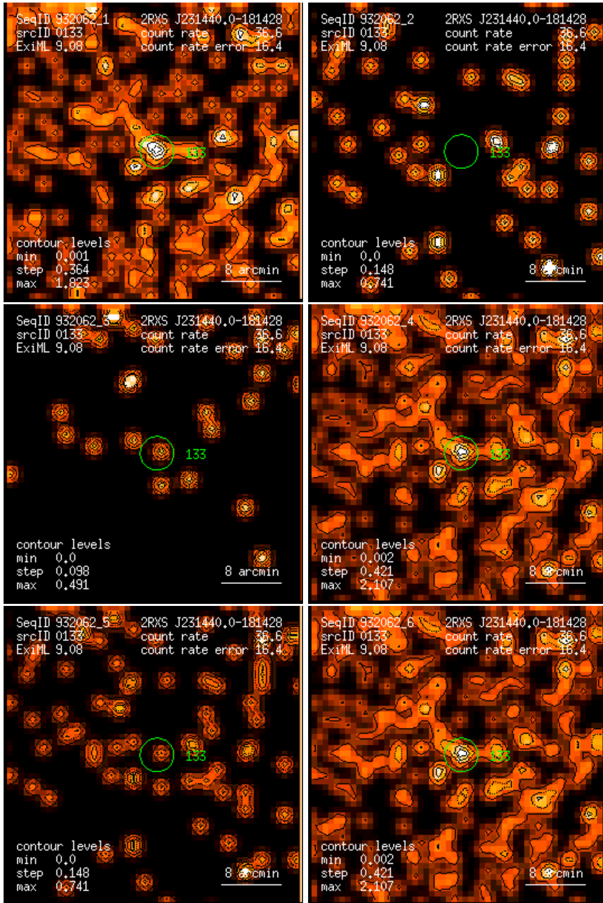
Figure 133: RASS 932062: detection 0133: band rate images, Gaussian filter: (1) PSPC channels 11 – 41, (2) 52 – 90, (3) 91 – 201, (4) 11 – 235, (5) 52 – 201, (6) 11 – 201. Broad band rates in counts/ks. Band rate contour levels in counts/ks/arcmin 2 .
