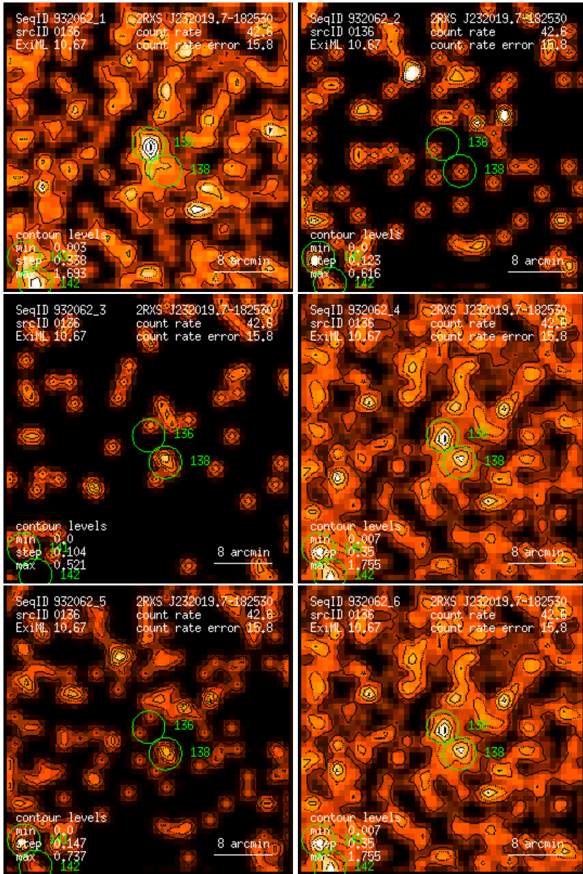
Figure 136: RASS 932062: detection 0136: band rate images, Gaussian filter: (1) PSPC channels 11 – 41, (2) 52 – 90, (3) 91 – 201, (4) 11 – 235, (5) 52 – 201, (6) 11 – 201. Broad band rates in counts/ks. Band rate contour levels in counts/ks/arcmin 2 .
