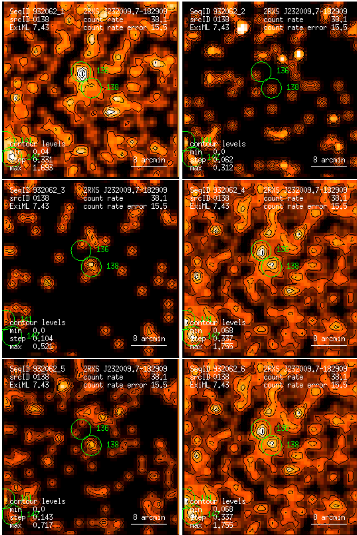
Figure 138: RASS 932062: detection 0138: band rate images, Gaussian filter: (1) PSPC channels 11 – 41, (2) 52 – 90, (3) 91 – 201, (4) 11 – 235, (5) 52 – 201, (6) 11 – 201. Broad band rates in counts/ks. Band rate contour levels in counts/ks/arcmin 2 .
