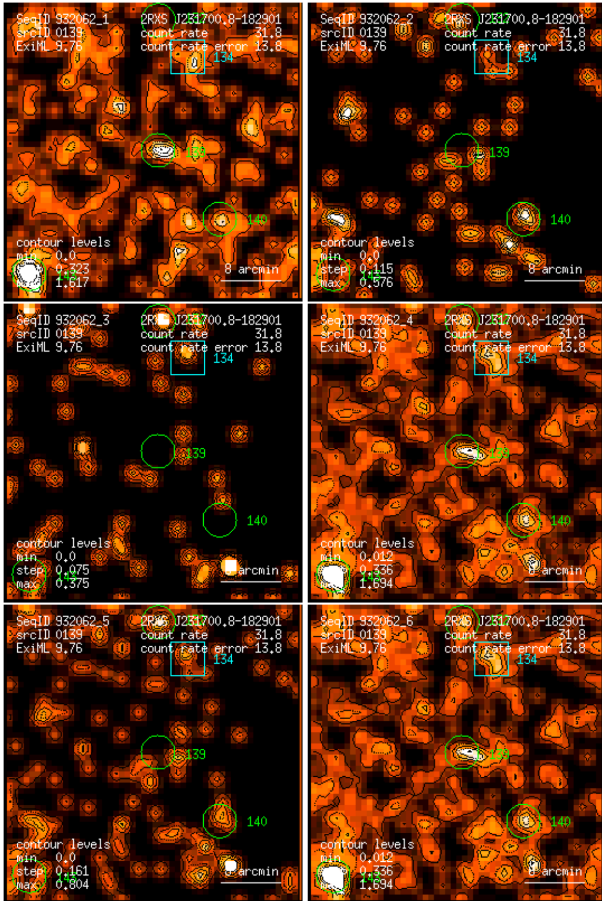
Figure 139: RASS 932062: detection 0139: band rate images, Gaussian filter: (1) PSPC channels 11 – 41, (2) 52 – 90, (3) 91 – 201, (4) 11 – 235, (5) 52 – 201, (6) 11 – 201. Broad band rates in counts/ks. Band rate contour levels in counts/ks/arcmin 2 .
