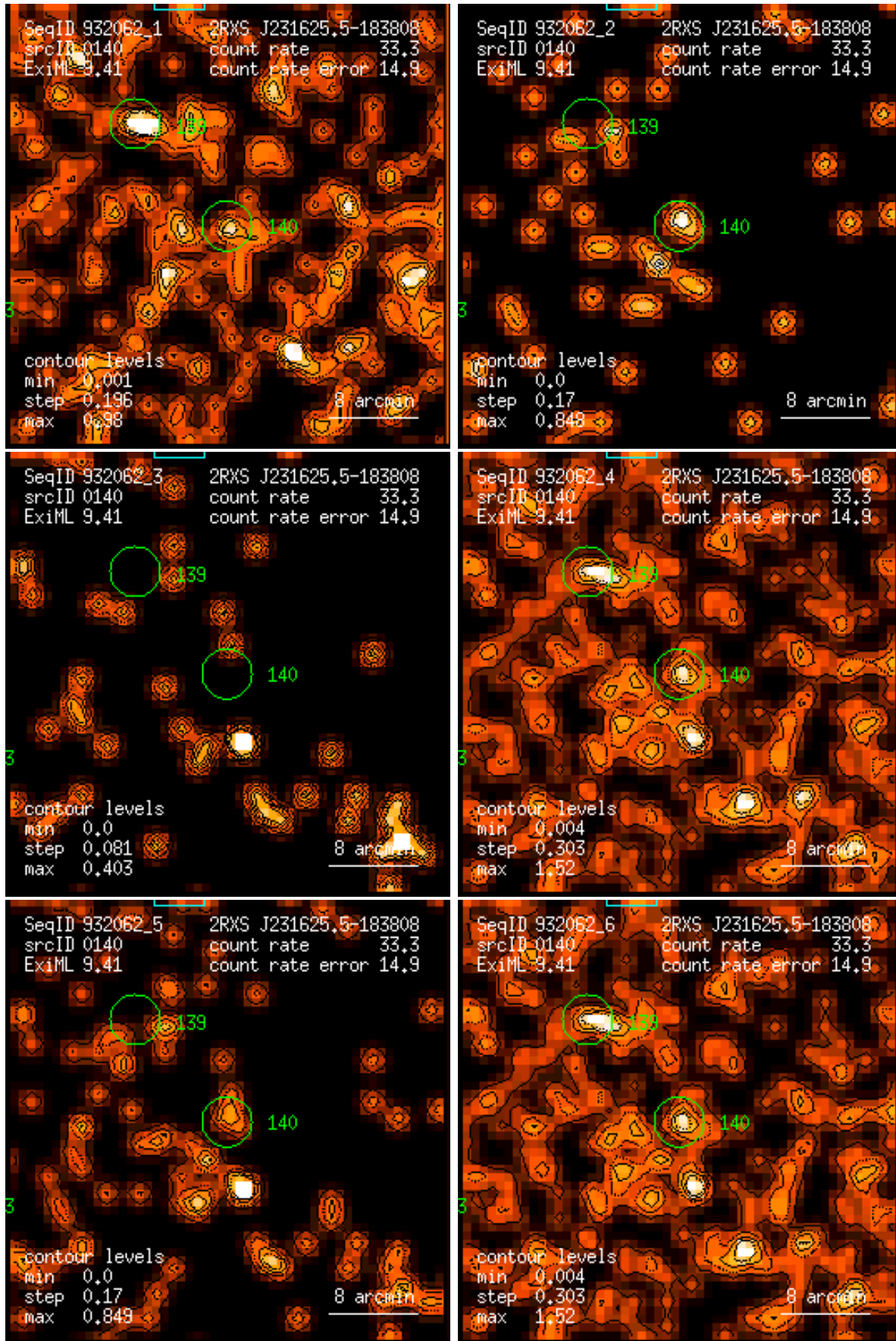
Figure 140: RASS 932062: detection 0140: band rate images, Gaussian filter: (1) PSPC channels 11 – 41, (2) 52 – 90, (3) 91 – 201, (4) 11 – 235, (5) 52 – 201, (6) 11 – 201. Broad band rates in counts/ks. Band rate contour levels in counts/ks/arcmin 2 .
