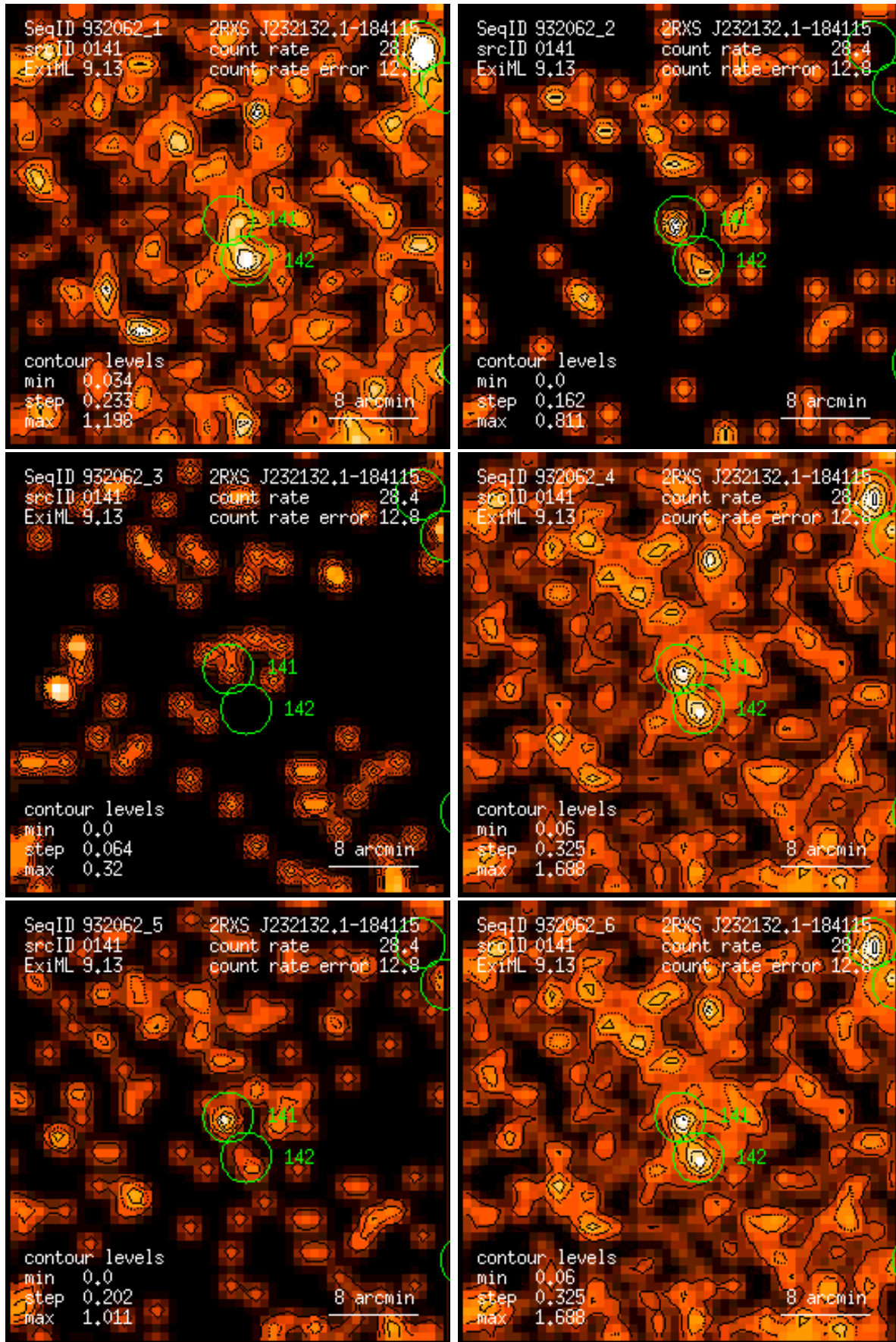
Figure 141: RASS 932062: detection 0141: band rate images, Gaussian filter: (1) PSPC channels 11 – 41, (2) 52 – 90, (3) 91 – 201, (4) 11 – 235, (5) 52 – 201, (6) 11 – 201. Broad band rates in counts/ks. Band rate contour levels in counts/ks/arcmin 2 .
