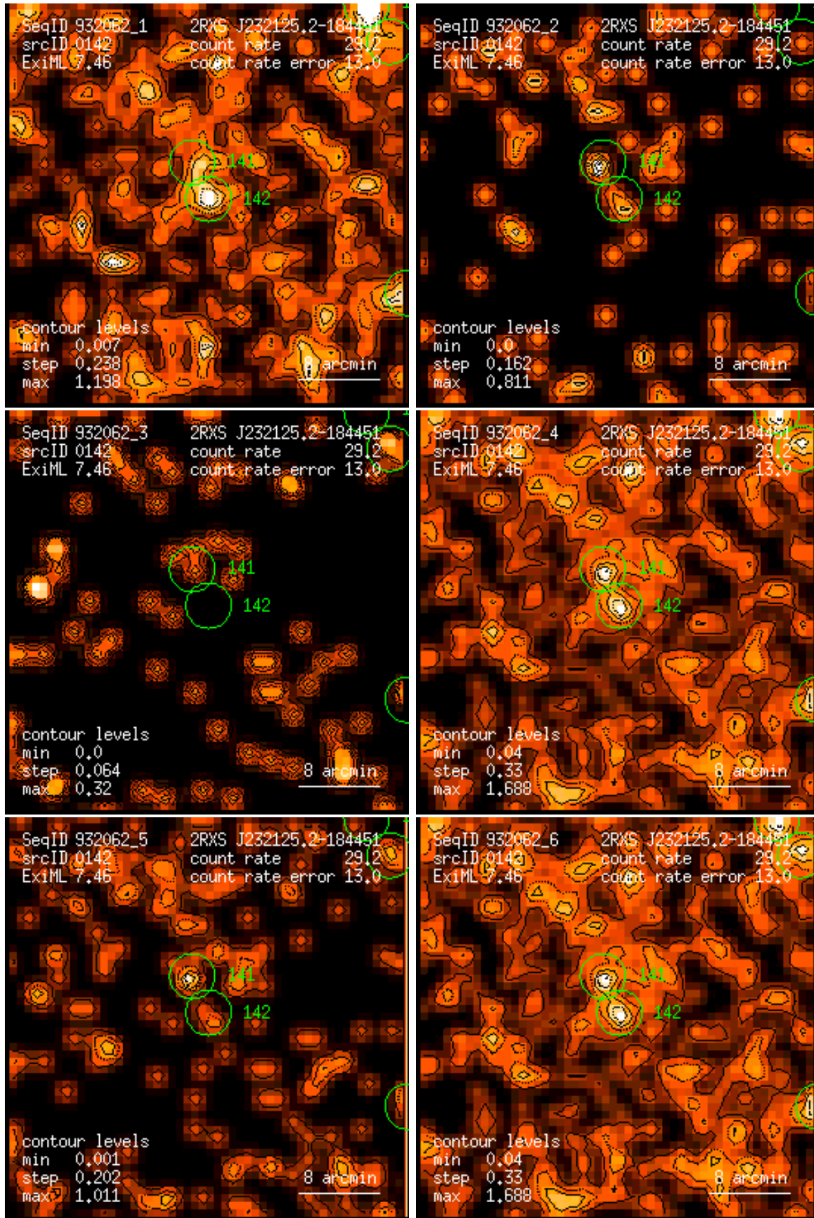
Figure 142: RASS 932062: detection 0142: band rate images, Gaussian filter: (1) PSPC channels 11 – 41, (2) 52 – 90, (3) 91 – 201, (4) 11 – 235, (5) 52 – 201, (6) 11 – 201. Broad band rates in counts/ks. Band rate contour levels in counts/ks/arcmin 2 .
