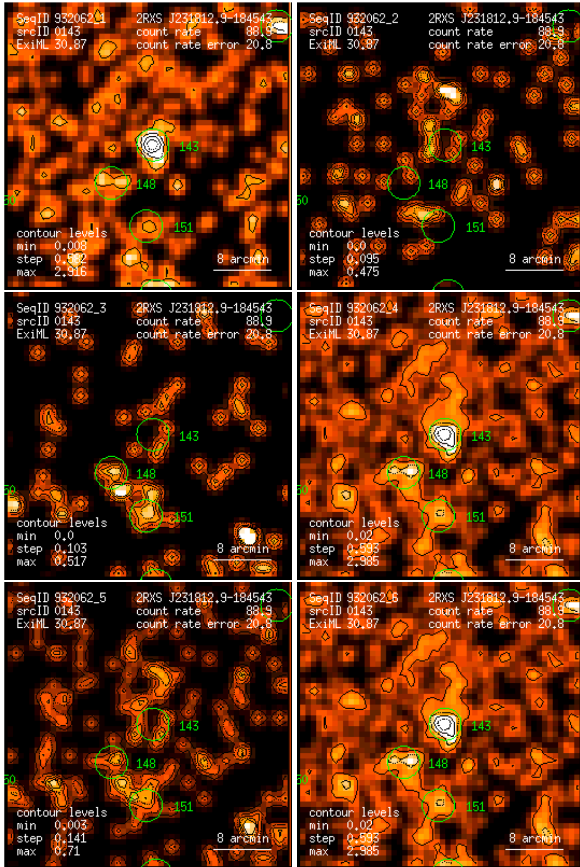
Figure 143: RASS 932062: detection 0143: band rate images, Gaussian filter: (1) PSPC channels 11 – 41, (2) 52 – 90, (3) 91 – 201, (4) 11 – 235, (5) 52 – 201, (6) 11 – 201. Broad band rates in counts/ks. Band rate contour levels in counts/ks/arcmin 2 .
