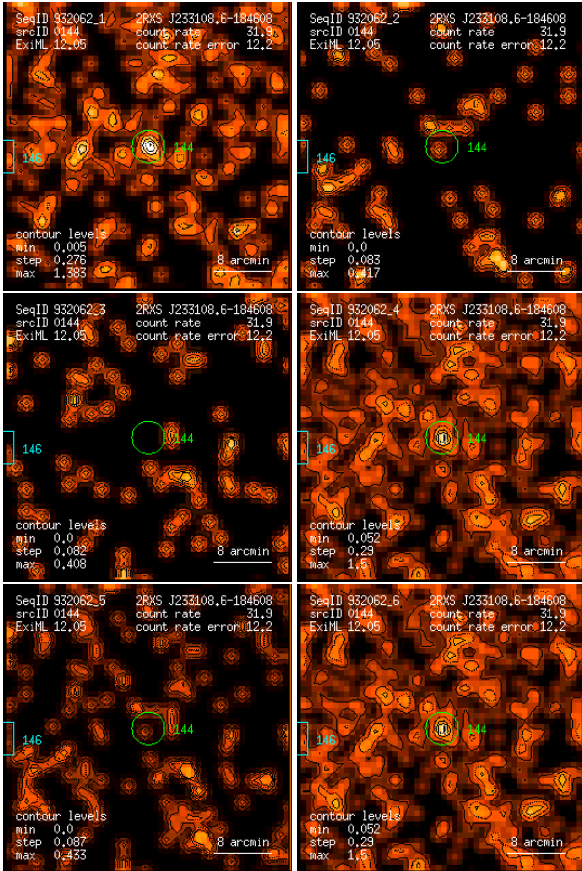
Figure 144: RASS 932062: detection 0144: band rate images, Gaussian filter: (1) PSPC channels 11 – 41, (2) 52 – 90, (3) 91 – 201, (4) 11 – 235, (5) 52 – 201, (6) 11 – 201. Broad band rates in counts/ks. Band rate contour levels in counts/ks/arcmin 2 .
