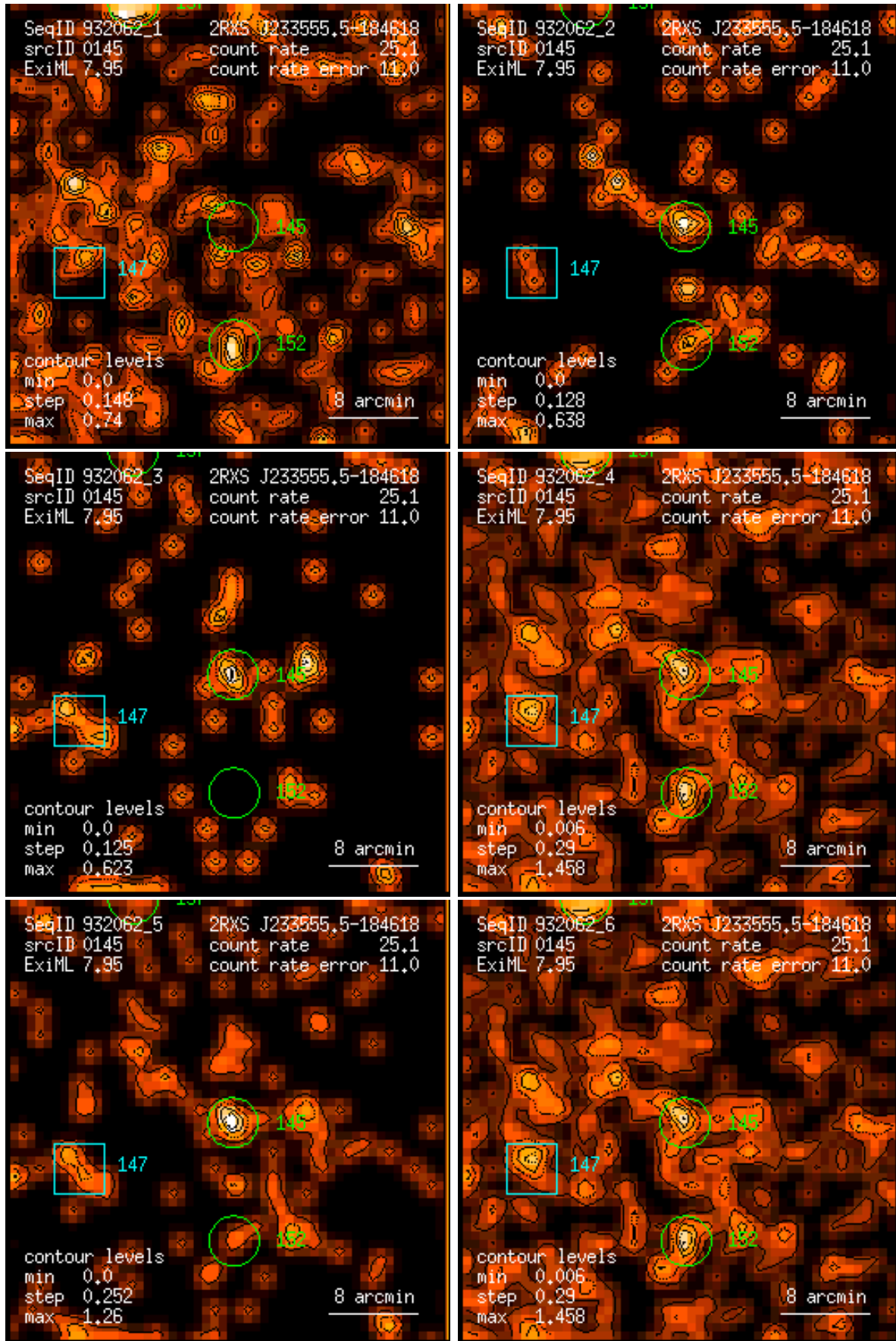
Figure 145: RASS 932062: detection 0145: band rate images, Gaussian filter: (1) PSPC channels 11 – 41, (2) 52 – 90, (3) 91 – 201, (4) 11 – 235, (5) 52 – 201, (6) 11 – 201. Broad band rates in counts/ks. Band rate contour levels in counts/ks/arcmin 2 .
