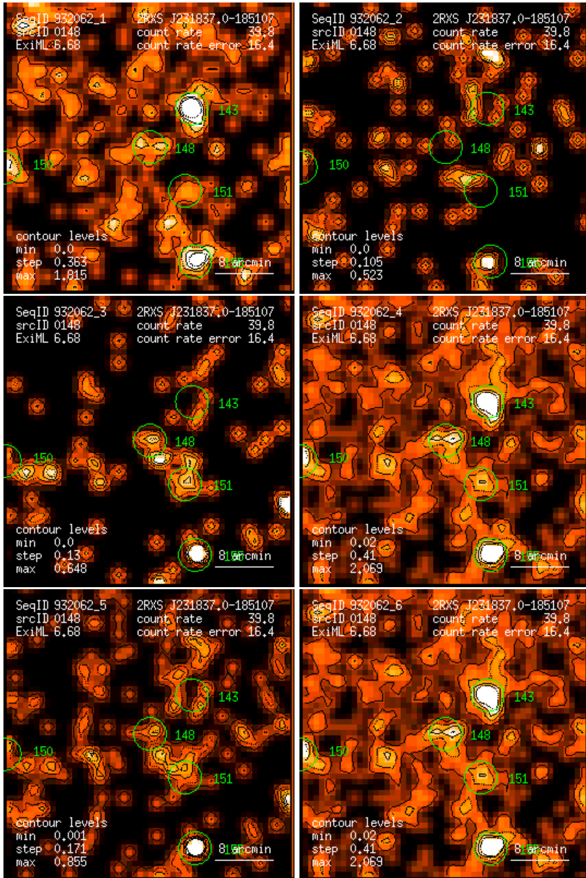
Figure 148: RASS 932062: detection 0148: band rate images, Gaussian filter: (1) PSPC channels 11 – 41, (2) 52 – 90, (3) 91 – 201, (4) 11 – 235, (5) 52 – 201, (6) 11 – 201. Broad band rates in counts/ks. Band rate contour levels in counts/ks/arcmin 2 .
