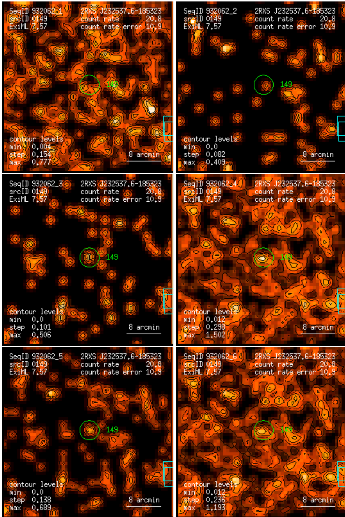
Figure 149: RASS 932062: detection 0149: band rate images, Gaussian filter: (1) PSPC channels 11 – 41, (2) 52 – 90, (3) 91 – 201, (4) 11 – 235, (5) 52 – 201, (6) 11 – 201. Broad band rates in counts/ks. Band rate contour levels in counts/ks/arcmin 2 .
