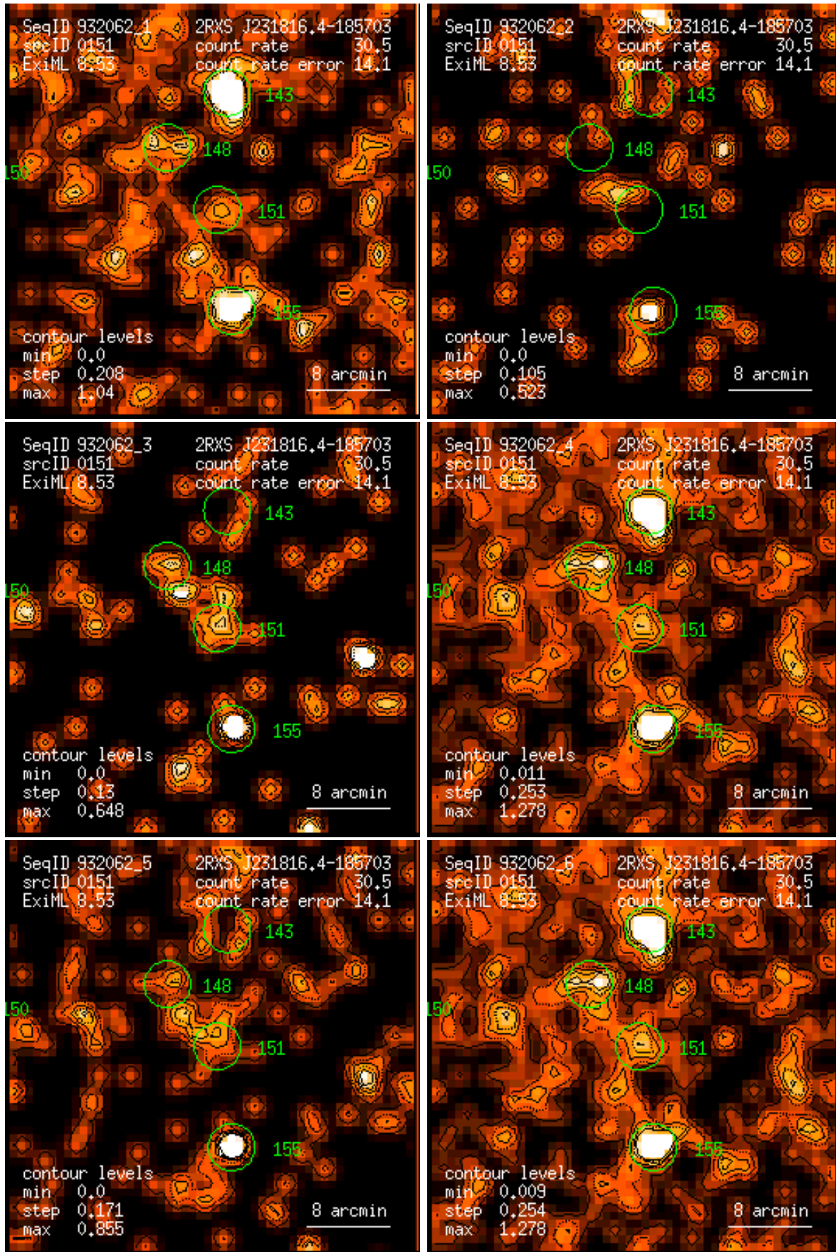
Figure 151: RASS 932062: detection 0151: band rate images, Gaussian filter: (1) PSPC channels 11 – 41, (2) 52 – 90, (3) 91 – 201, (4) 11 – 235, (5) 52 – 201, (6) 11 – 201. Broad band rates in counts/ks. Band rate contour levels in counts/ks/arcmin 2 .
