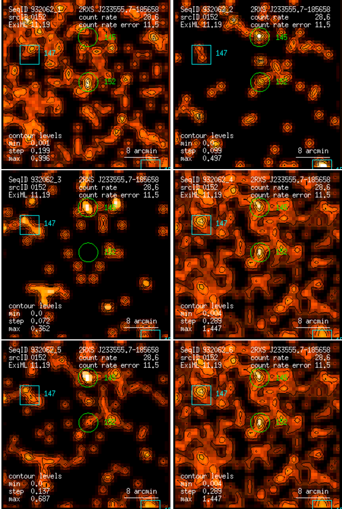
Figure 152: RASS 932062: detection 0152: band rate images, Gaussian filter: (1) PSPC channels 11 – 41, (2) 52 – 90, (3) 91 – 201, (4) 11 – 235, (5) 52 – 201, (6) 11 – 201. Broad band rates in counts/ks. Band rate contour levels in counts/ks/arcmin 2 .
