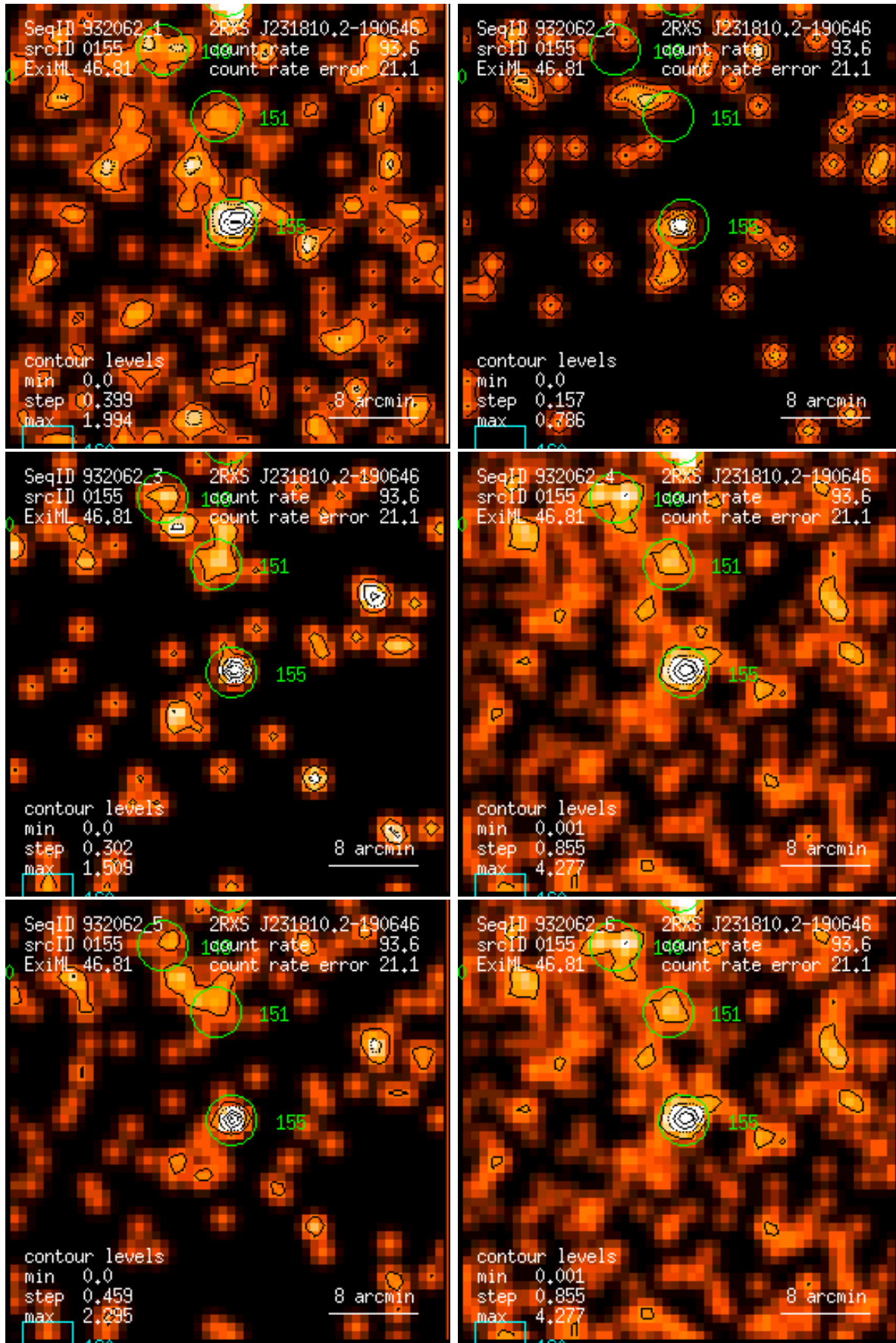
Figure 155: RASS 932062: detection 0155: band rate images, Gaussian filter: (1) PSPC channels 11 – 41, (2) 52 – 90, (3) 91 – 201, (4) 11 – 235, (5) 52 – 201, (6) 11 – 201. Broad band rates in counts/ks. Band rate contour levels in counts/ks/arcmin 2 .
