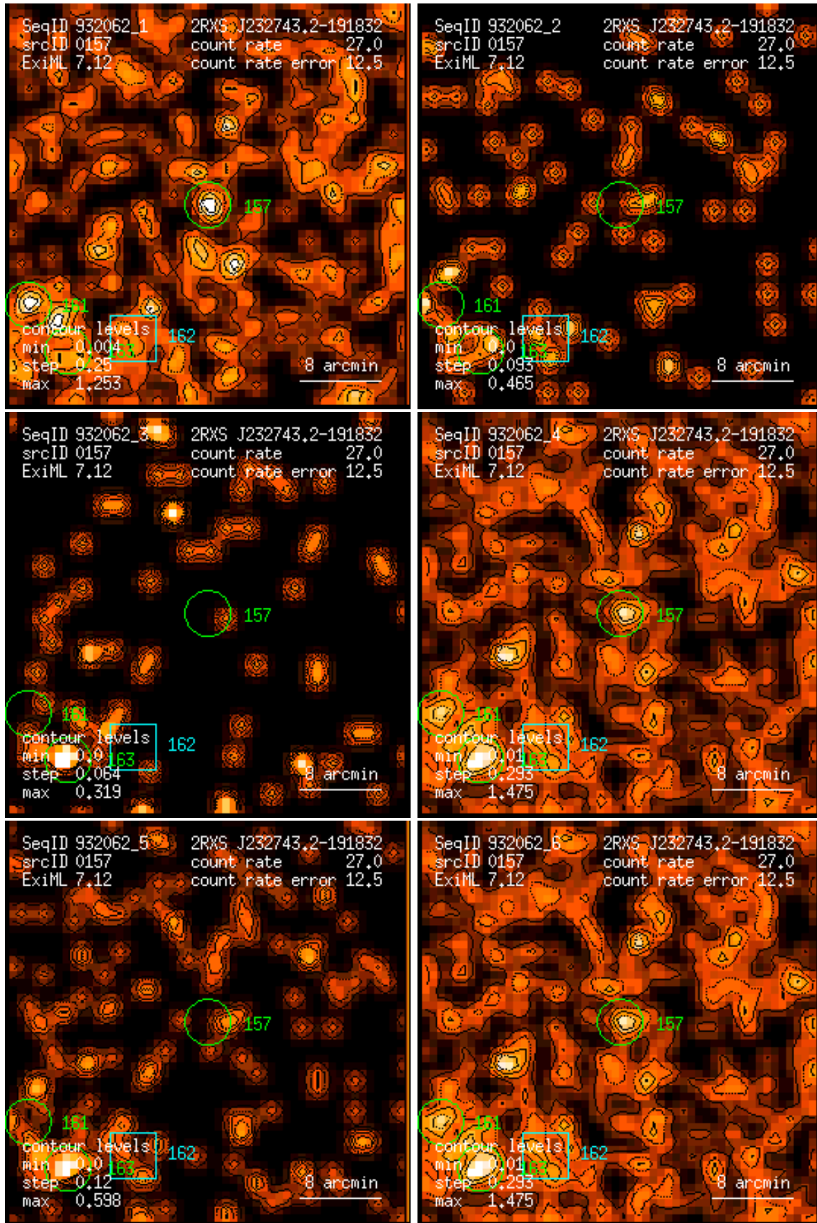
Figure 157: RASS 932062: detection 0157: band rate images, Gaussian filter: (1) PSPC channels 11 – 41, (2) 52 – 90, (3) 91 – 201, (4) 11 – 235, (5) 52 – 201, (6) 11 – 201. Broad band rates in counts/ks. Band rate contour levels in counts/ks/arcmin 2 .
