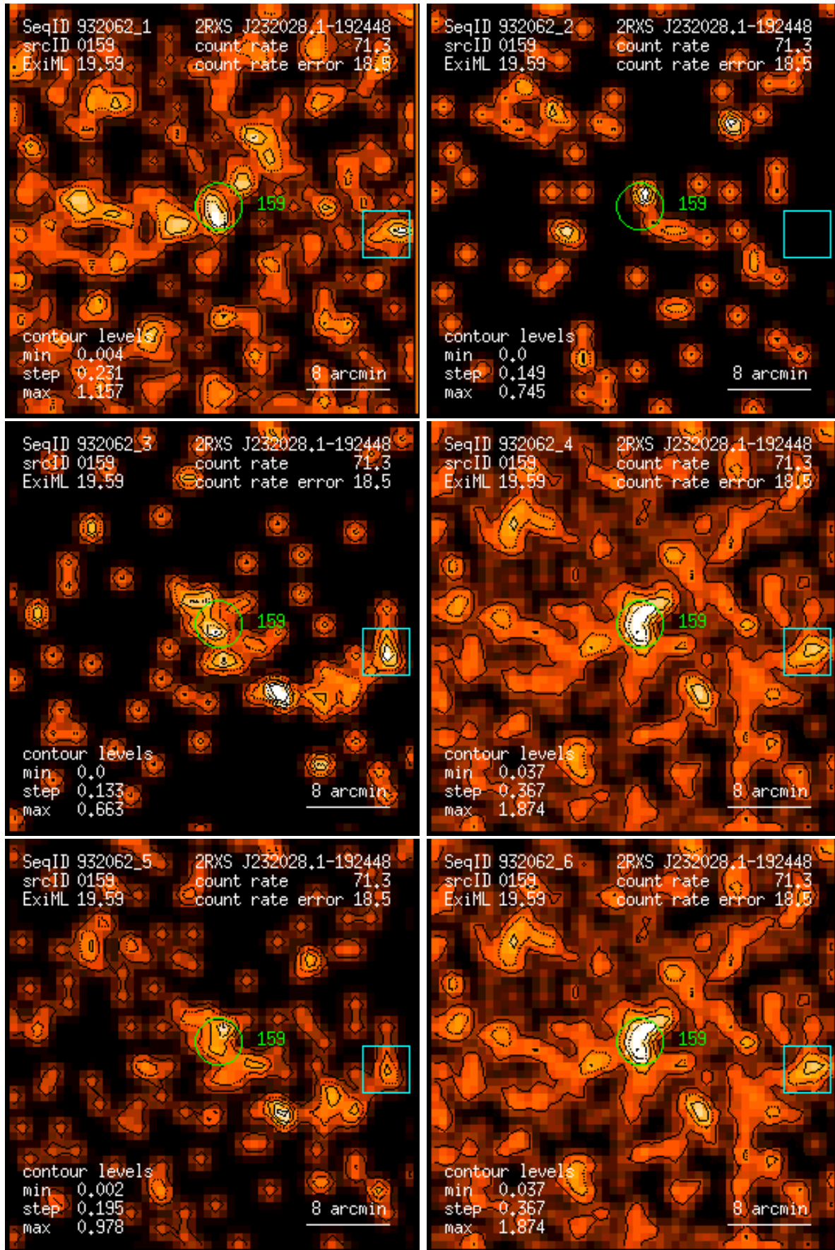
Figure 159: RASS 932062: detection 0159: band rate images, Gaussian filter: (1) PSPC channels 11 – 41, (2) 52 – 90, (3) 91 – 201, (4) 11 – 235, (5) 52 – 201, (6) 11 – 201. Broad band rates in counts/ks. Band rate contour levels in counts/ks/arcmin 2 .
