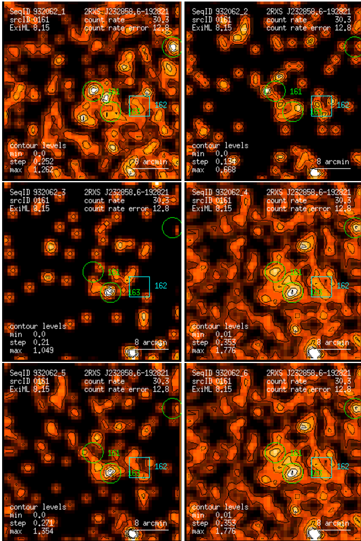
Figure 161: RASS 932062: detection 0161: band rate images, Gaussian filter: (1) PSPC channels 11 – 41, (2) 52 – 90, (3) 91 – 201, (4) 11 – 235, (5) 52 – 201, (6) 11 – 201. Broad band rates in counts/ks. Band rate contour levels in counts/ks/arcmin 2 .
