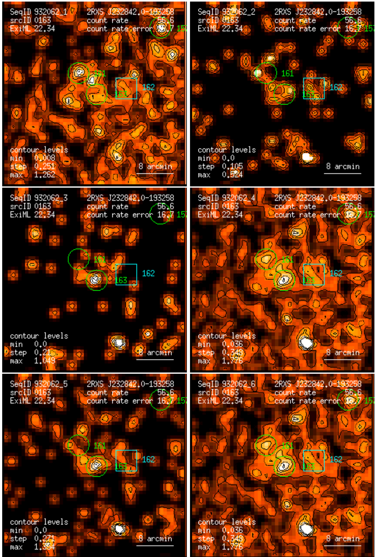
Figure 163: RASS 932062: detection 0163: band rate images, Gaussian filter: (1) PSPC channels 11 – 41, (2) 52 – 90, (3) 91 – 201, (4) 11 – 235, (5) 52 – 201, (6) 11 – 201. Broad band rates in counts/ks. Band rate contour levels in counts/ks/arcmin 2 .
