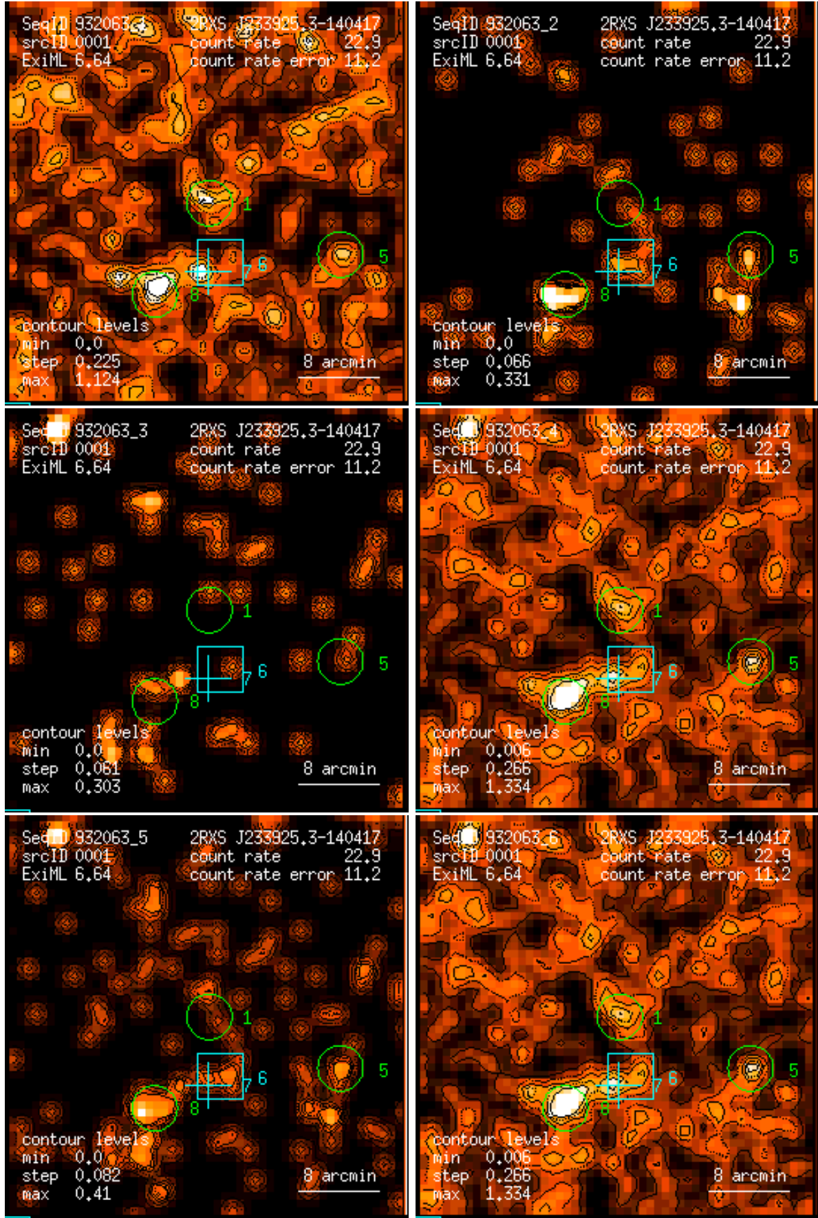
Figure 1: RASS 932063: detection 0001: band rate images, Gaussian filter: (1) PSPC channels 11 – 41, (2) 52 – 90, (3) 91 – 201, (4) 11 – 235, (5) 52 – 201, (6) 11 – 201. Broad band rates in counts/ks. Band rate contour levels in counts/ks/arcmin 2 .
