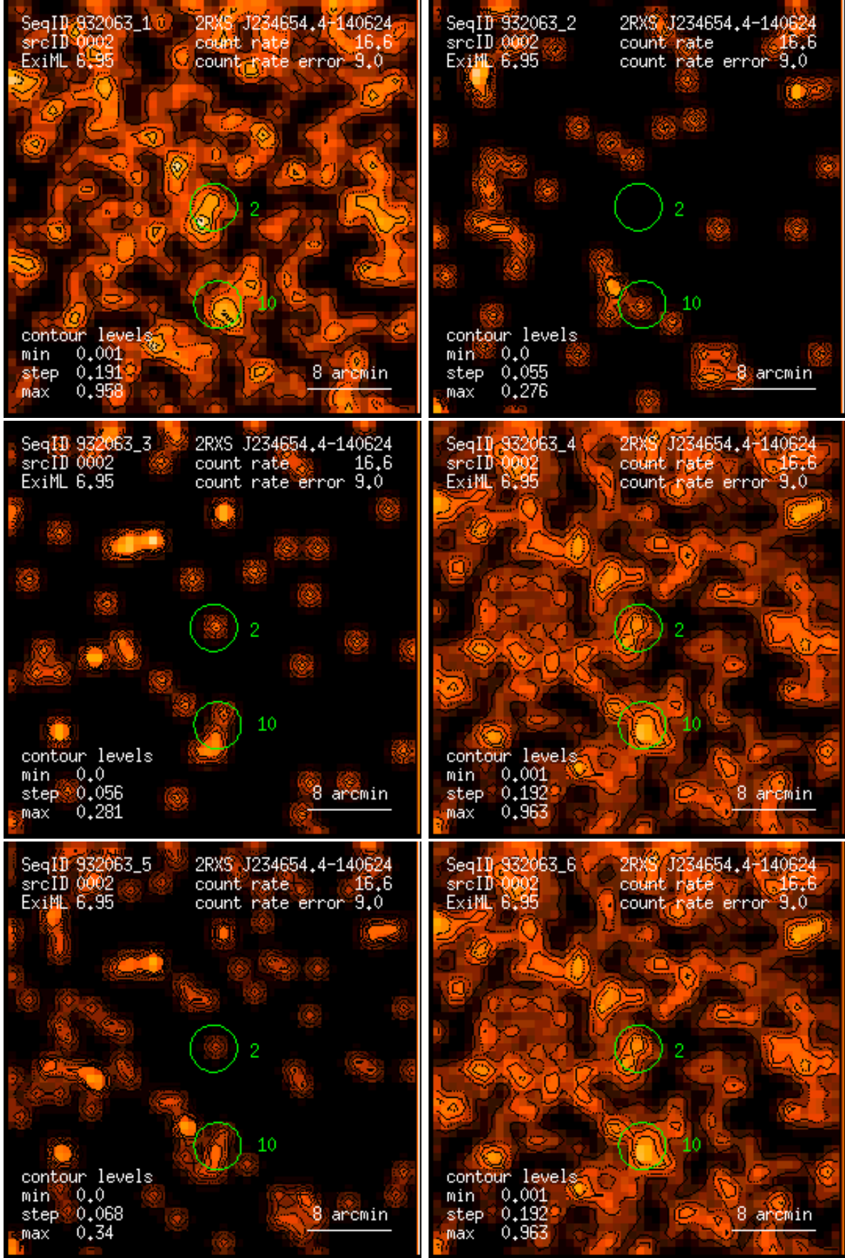
Figure 2: RASS 932063: detection 0002: band rate images, Gaussian filter: (1) PSPC channels 11 – 41, (2) 52 – 90, (3) 91 – 201, (4) 11 – 235, (5) 52 – 201, (6) 11 – 201. Broad band rates in counts/ks. Band rate contour levels in counts/ks/arcmin 2 .
