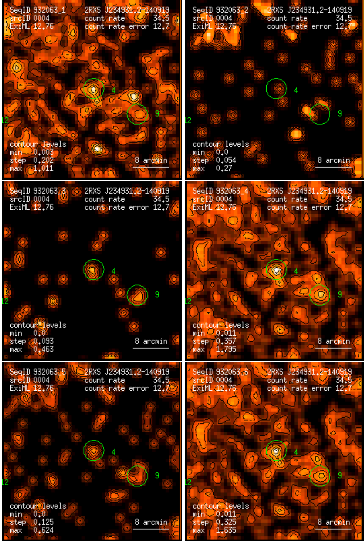
Figure 4: RASS 932063: detection 0004: band rate images, Gaussian filter: (1) PSPC channels 11 – 41, (2) 52 – 90, (3) 91 – 201, (4) 11 – 235, (5) 52 – 201, (6) 11 – 201. Broad band rates in counts/ks. Band rate contour levels in counts/ks/arcmin 2 .
