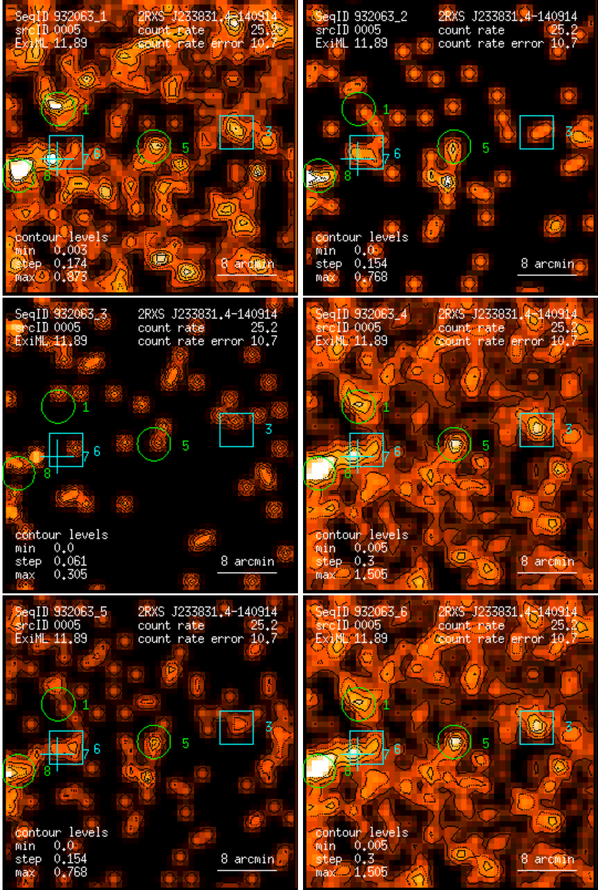
Figure 5: RASS 932063: detection 0005: band rate images, Gaussian filter: (1) PSPC channels 11 – 41, (2) 52 – 90, (3) 91 – 201, (4) 11 – 235, (5) 52 – 201, (6) 11 – 201. Broad band rates in counts/ks. Band rate contour levels in counts/ks/arcmin 2 .
