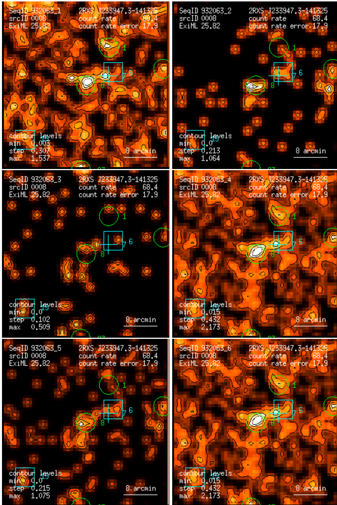
Figure 8: RASS 932063: detection 0008: band rate images, Gaussian filter: (1) PSPC channels 11 – 41, (2) 52 – 90, (3) 91 – 201, (4) 11 – 235, (5) 52 – 201, (6) 11 – 201. Broad band rates in counts/ks. Band rate contour levels in counts/ks/arcmin 2 .
