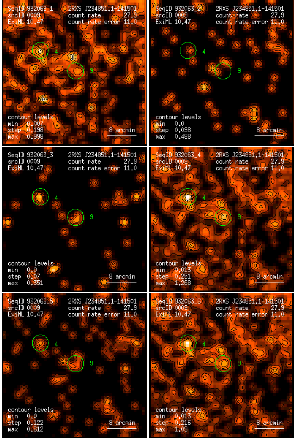
Figure 9: RASS 932063: detection 0009: band rate images, Gaussian filter: (1) PSPC channels 11 – 41, (2) 52 – 90, (3) 91 – 201, (4) 11 – 235, (5) 52 – 201, (6) 11 – 201. Broad band rates in counts/ks. Band rate contour levels in counts/ks/arcmin 2 .
