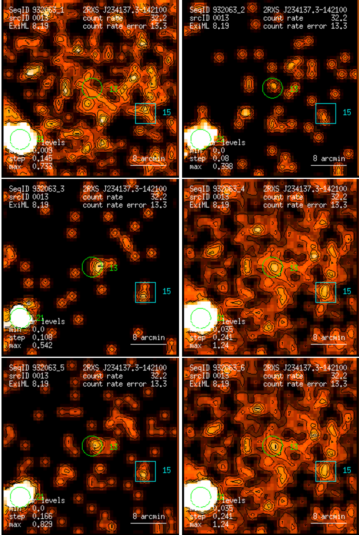
Figure 13: RASS 932063: detection 0013: band rate images, Gaussian filter: (1) PSPC channels 11 – 41, (2) 52 – 90, (3) 91 – 201, (4) 11 – 235, (5) 52 – 201, (6) 11 – 201. Broad band rates in counts/ks. Band rate contour levels in counts/ks/arcmin 2 .
