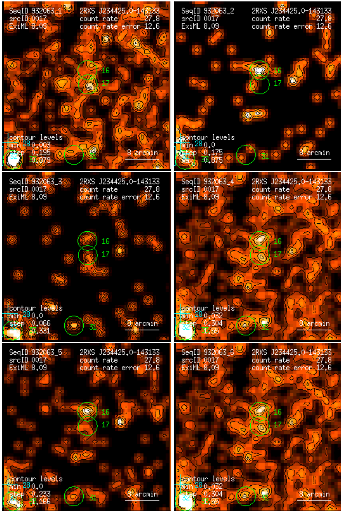
Figure 17: RASS 932063: detection 0017: band rate images, Gaussian filter: (1) PSPC channels 11 – 41, (2) 52 – 90, (3) 91 – 201, (4) 11 – 235, (5) 52 – 201, (6) 11 – 201. Broad band rates in counts/ks. Band rate contour levels in counts/ks/arcmin 2 .
