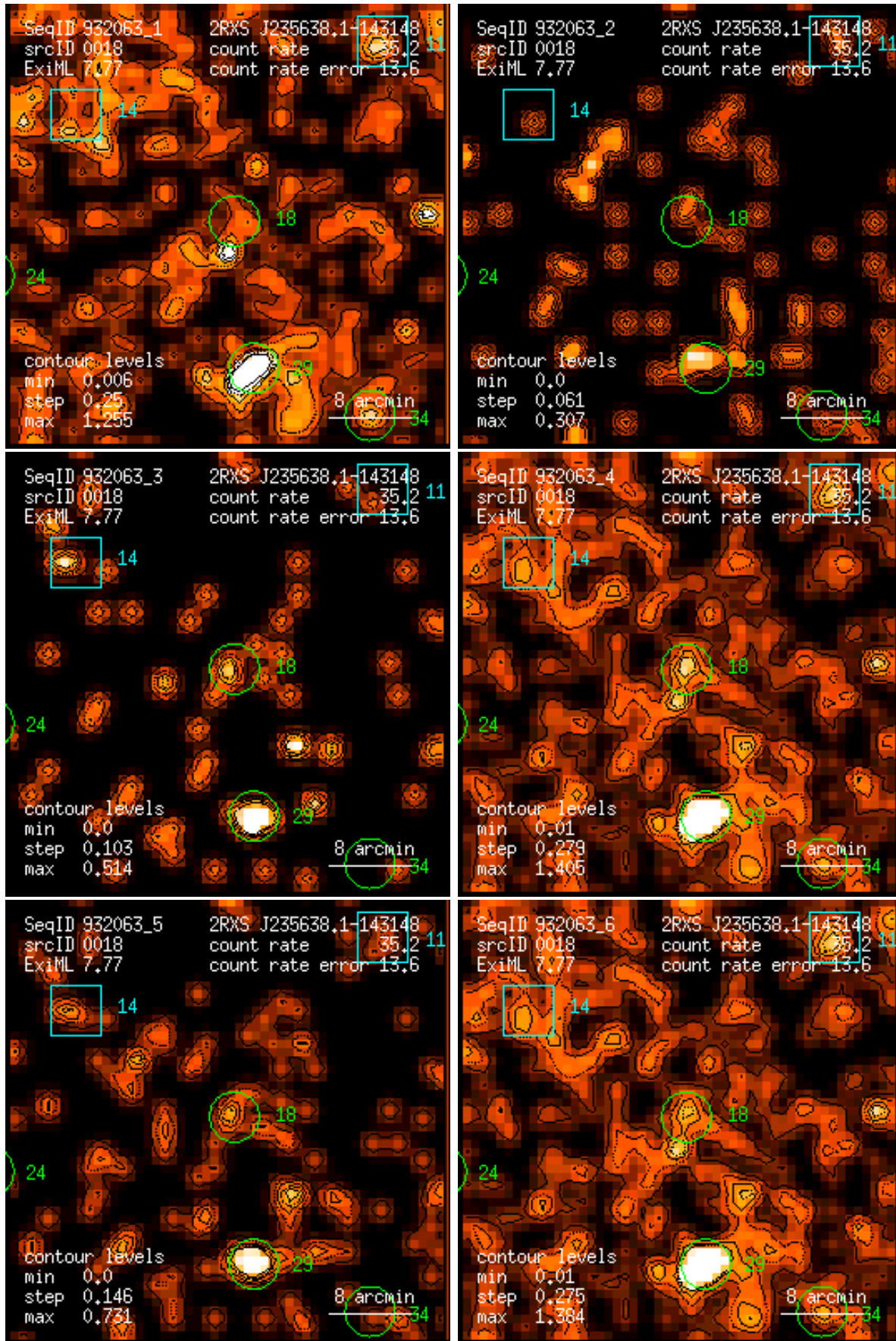
Figure 18: RASS 932063: detection 0018: band rate images, Gaussian filter: (1) PSPC channels 11 – 41, (2) 52 – 90, (3) 91 – 201, (4) 11 – 235, (5) 52 – 201, (6) 11 – 201. Broad band rates in counts/ks. Band rate contour levels in counts/ks/arcmin 2 .
