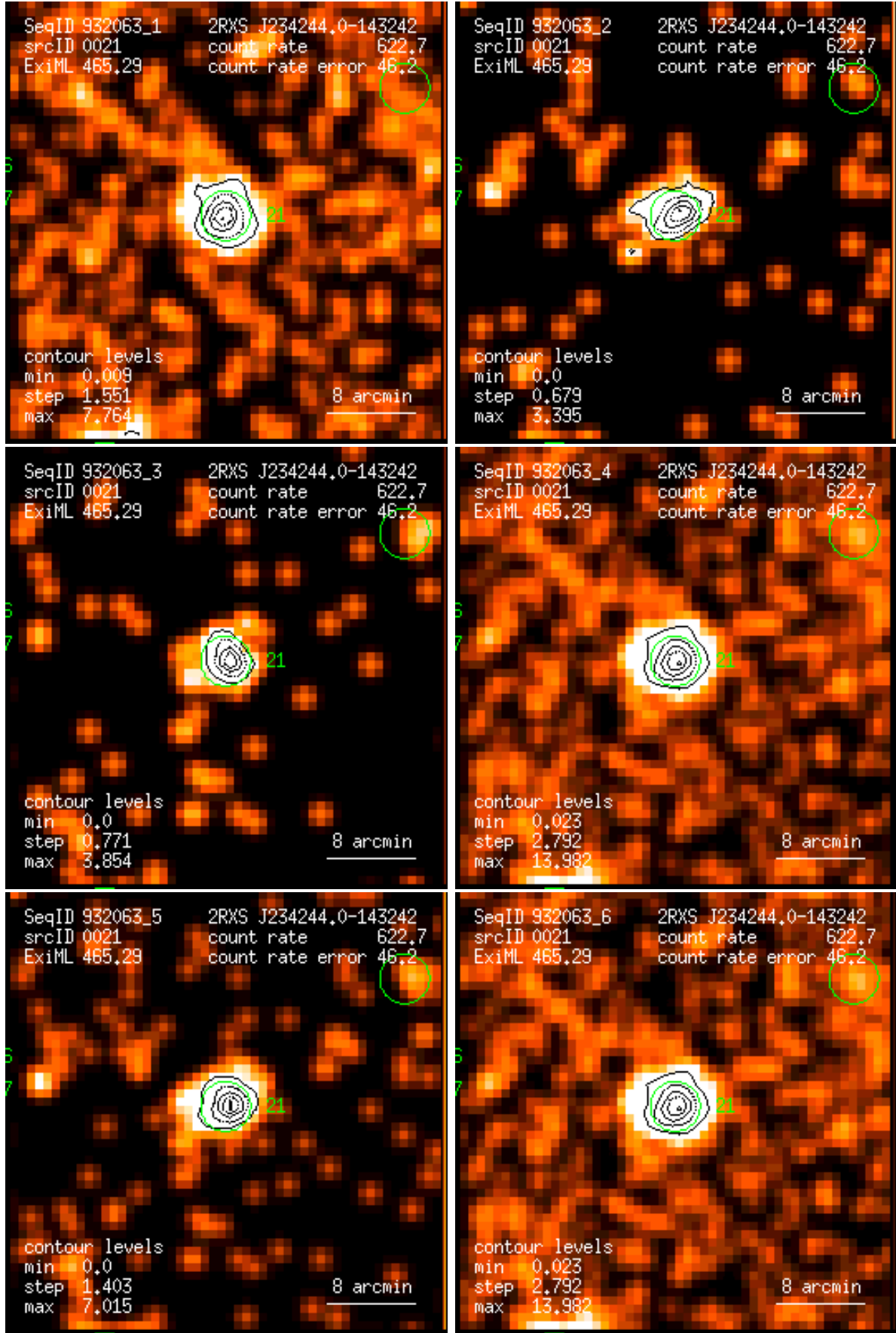
Figure 21: RASS 932063: detection 0021: band rate images, Gaussian filter: (1) PSPC channels 11 – 41, (2) 52 – 90, (3) 91 – 201, (4) 11 – 235, (5) 52 – 201, (6) 11 – 201. Broad band rates in counts/ks. Band rate contour levels in counts/ks/arcmin 2 .
