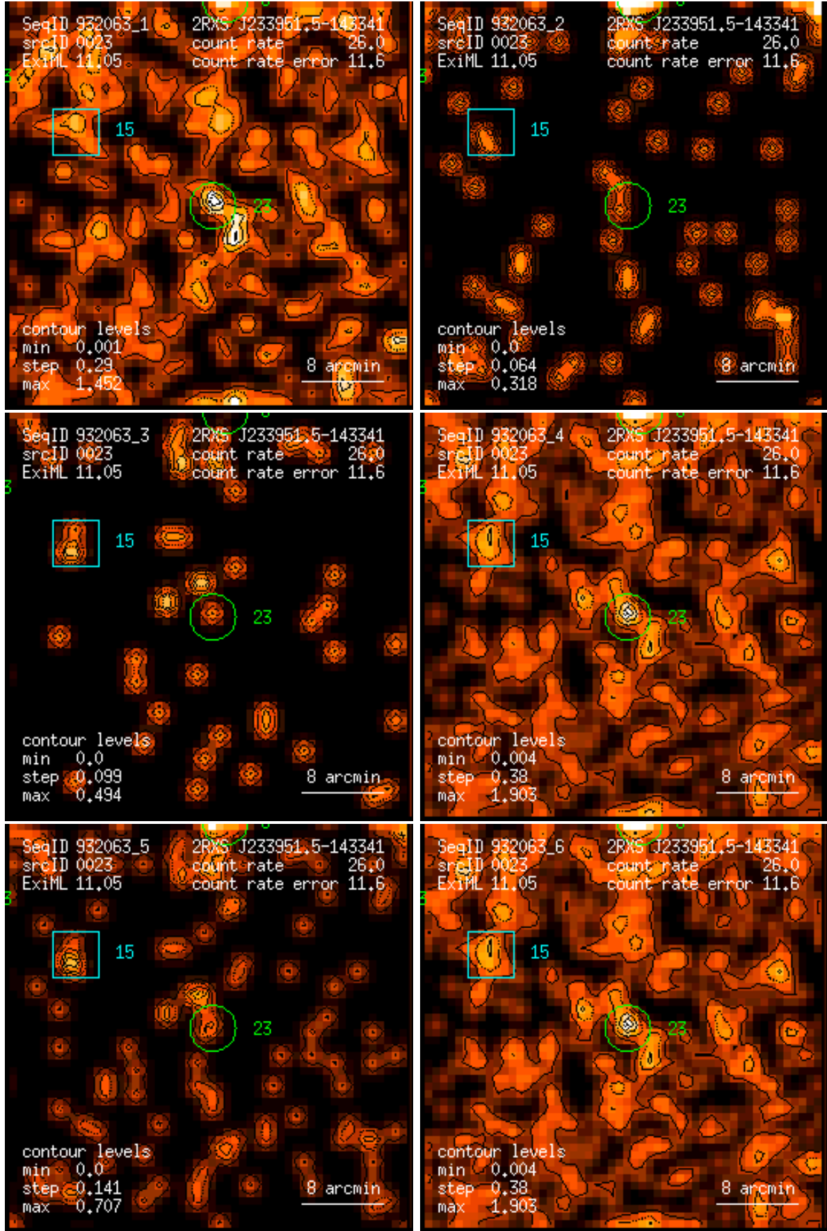
Figure 23: RASS 932063: detection 0023: band rate images, Gaussian filter: (1) PSPC channels 11 – 41, (2) 52 – 90, (3) 91 – 201, (4) 11 – 235, (5) 52 – 201, (6) 11 – 201. Broad band rates in counts/ks. Band rate contour levels in counts/ks/arcmin 2 .
