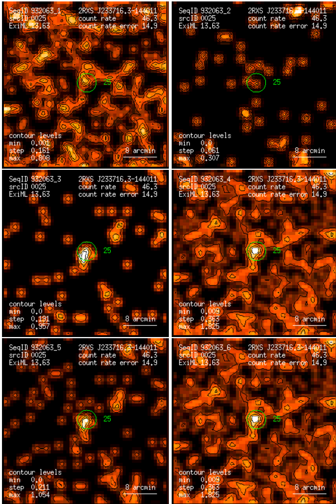
Figure 25: RASS 932063: detection 0025: band rate images, Gaussian filter: (1) PSPC channels 11 – 41, (2) 52 – 90, (3) 91 – 201, (4) 11 – 235, (5) 52 – 201, (6) 11 – 201. Broad band rates in counts/ks. Band rate contour levels in counts/ks/arcmin 2 .
