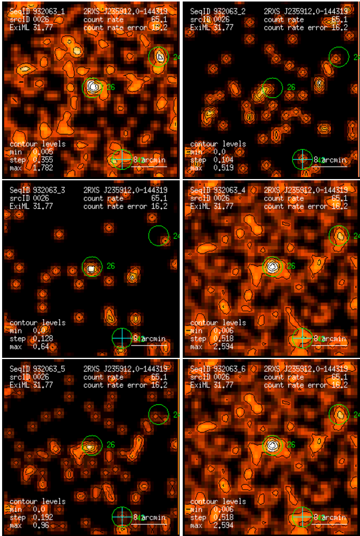
Figure 26: RASS 932063: detection 0026: band rate images, Gaussian filter: (1) PSPC channels 11 – 41, (2) 52 – 90, (3) 91 – 201, (4) 11 – 235, (5) 52 – 201, (6) 11 – 201. Broad band rates in counts/ks. Band rate contour levels in counts/ks/arcmin 2 .
