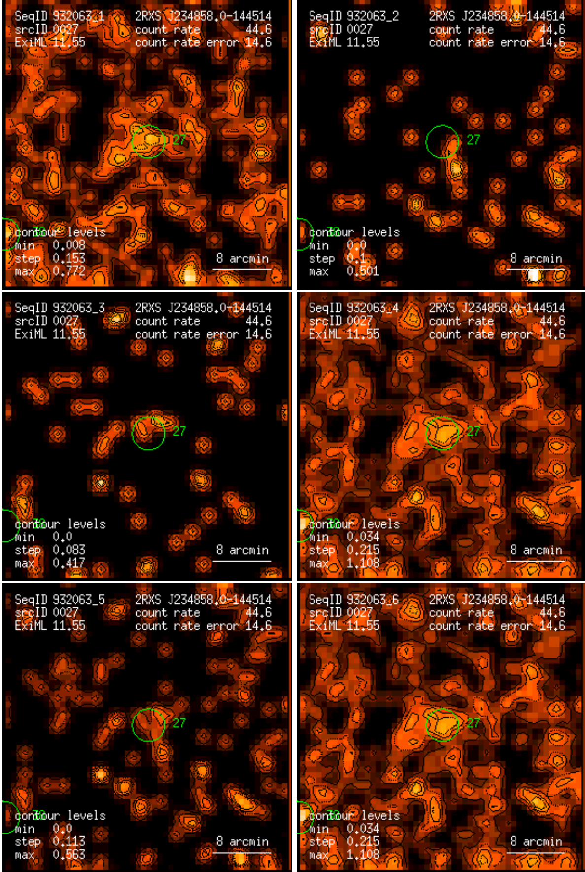
Figure 27: RASS 932063: detection 0027: band rate images, Gaussian filter: (1) PSPC channels 11 – 41, (2) 52 – 90, (3) 91 – 201, (4) 11 – 235, (5) 52 – 201, (6) 11 – 201. Broad band rates in counts/ks. Band rate contour levels in counts/ks/arcmin 2 .
