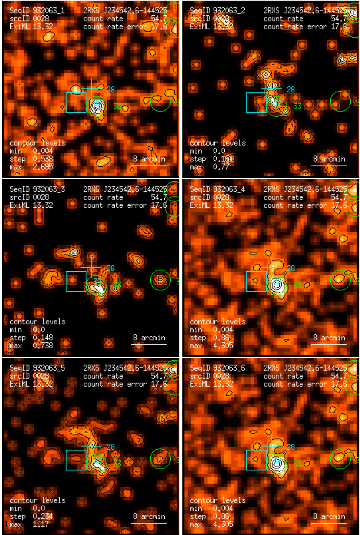
Figure 28: RASS 932063: detection 0028: band rate images, Gaussian filter: (1) PSPC channels 11 – 41, (2) 52 – 90, (3) 91 – 201, (4) 11 – 235, (5) 52 – 201, (6) 11 – 201. Broad band rates in counts/ks. Band rate contour levels in counts/ks/arcmin 2 .
