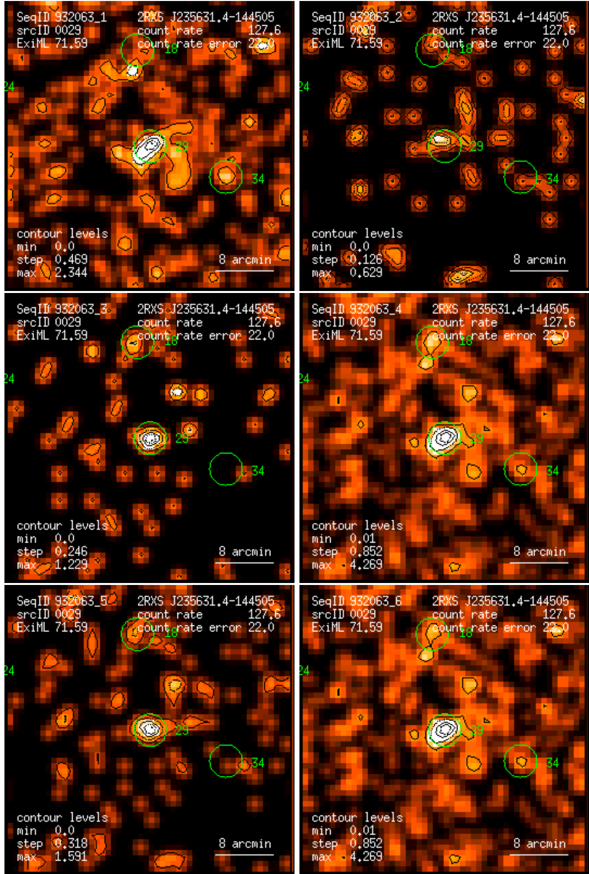
Figure 29: RASS 932063: detection 0029: band rate images, Gaussian filter: (1) PSPC channels 11 – 41, (2) 52 – 90, (3) 91 – 201, (4) 11 – 235, (5) 52 – 201, (6) 11 – 201. Broad band rates in counts/ks. Band rate contour levels in counts/ks/arcmin 2 .
